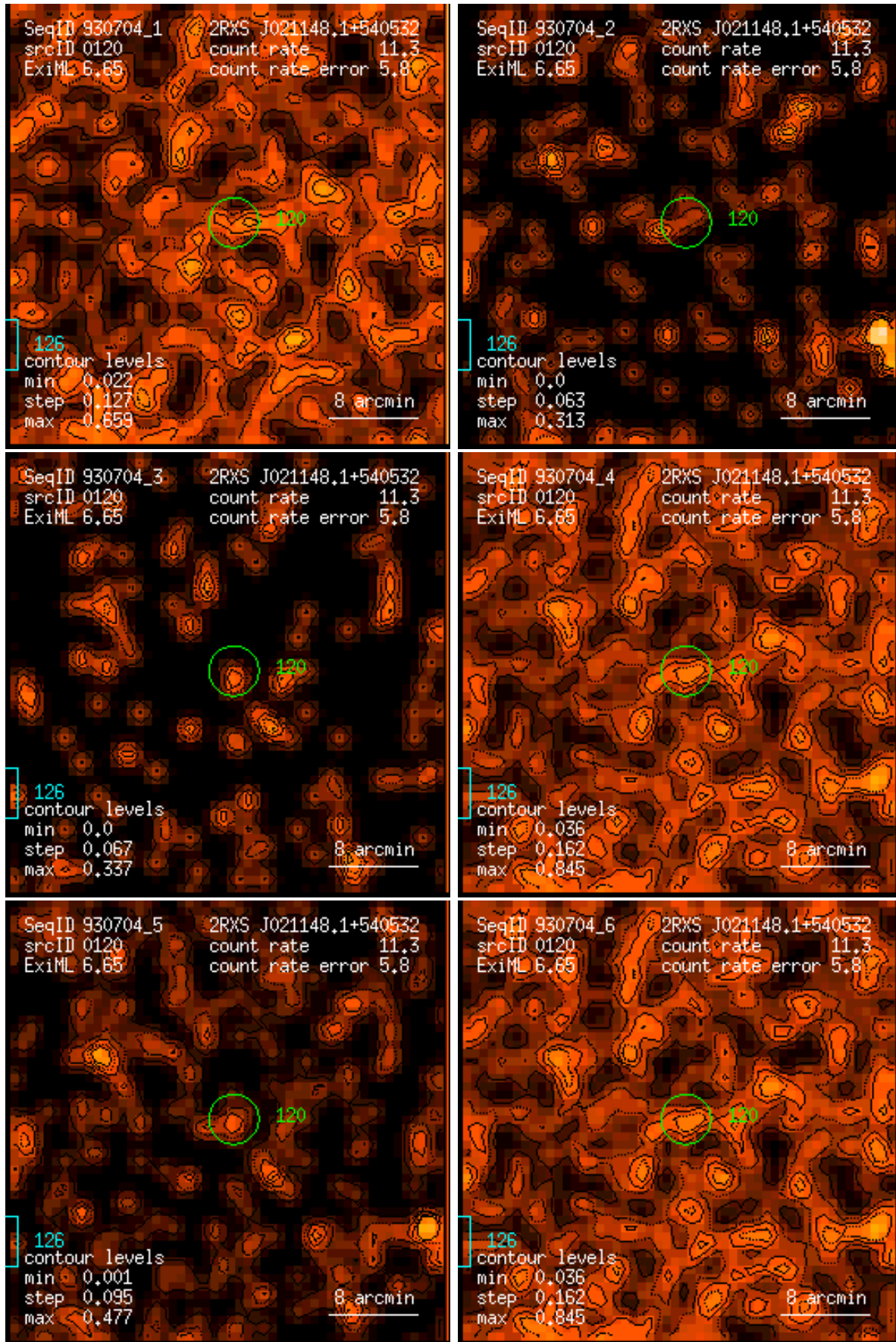
Figure 120: RASS 930704: detection 0120: band rate images, Gaussian filter: (1) PSPC channels 11 – 41, (2) 52 – 90, (3) 91 – 201, (4) 11 – 235, (5) 52 – 201, (6) 11 – 201. Broad band rates in counts/ks. Band rate contour levels in counts/ks/arcmin 2 .
