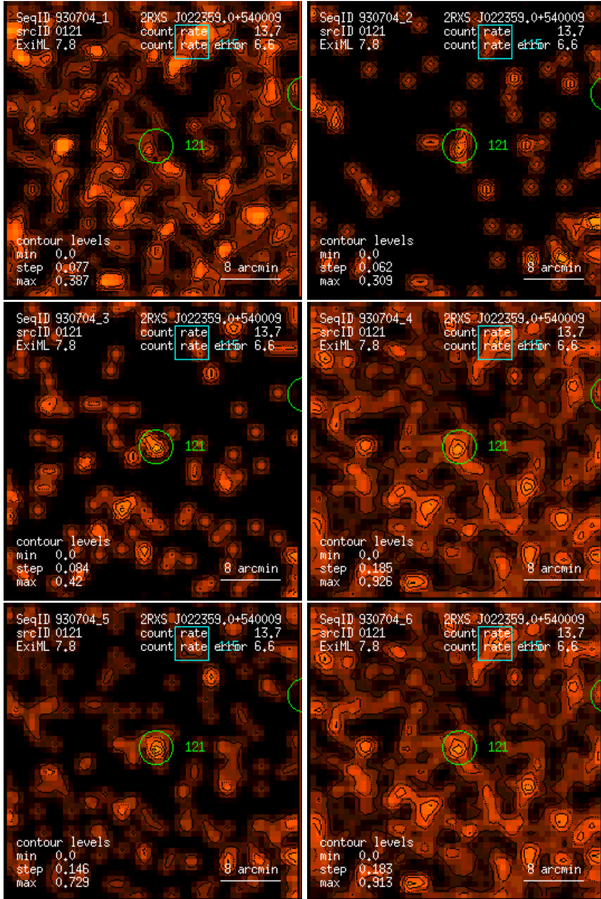
Figure 121: RASS 930704: detection 0121: band rate images, Gaussian filter: (1) PSPC channels 11 – 41, (2) 52 – 90, (3) 91 – 201, (4) 11 – 235, (5) 52 – 201, (6) 11 – 201. Broad band rates in counts/ks. Band rate contour levels in counts/ks/arcmin 2 .
