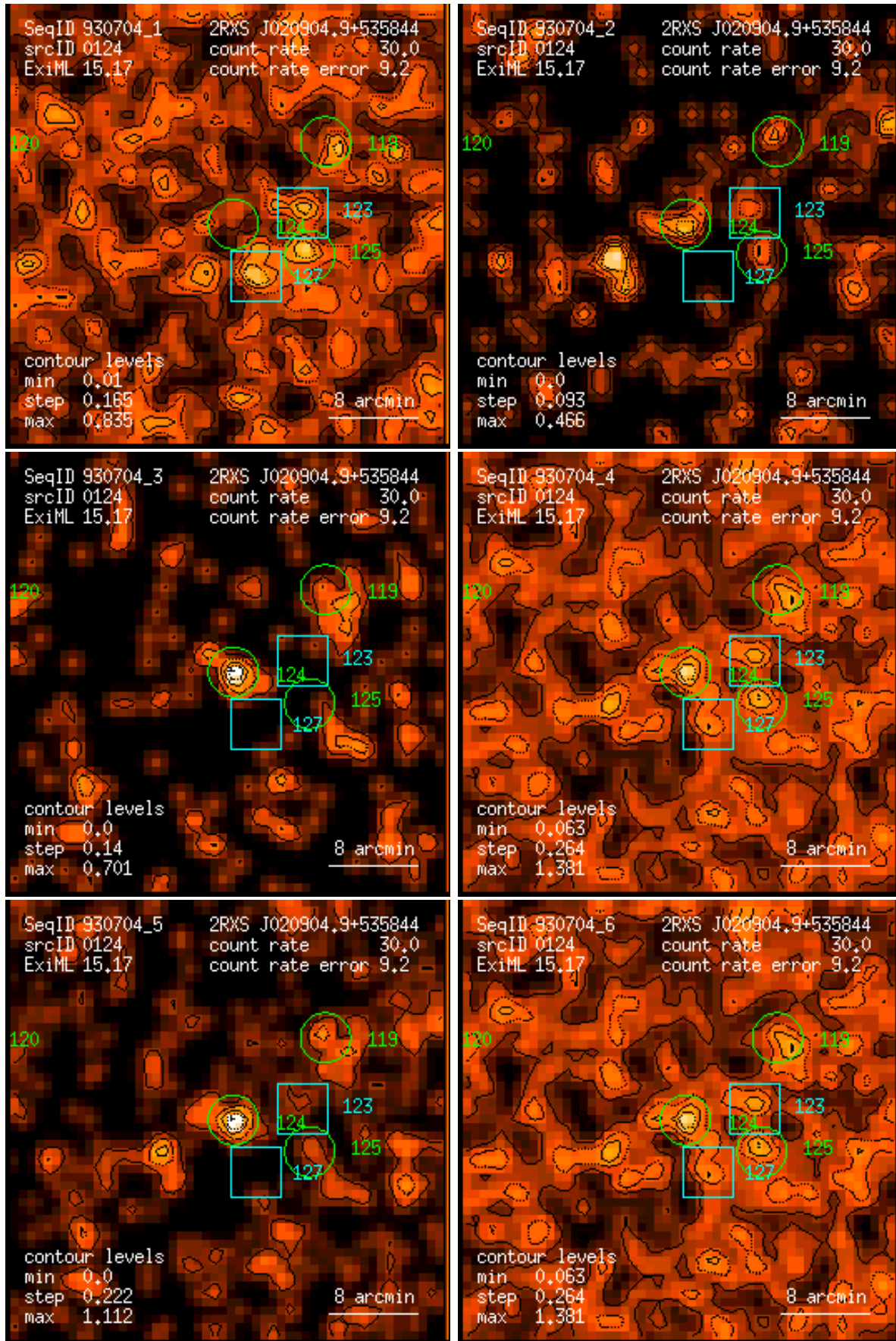
Figure 124: RASS 930704: detection 0124: band rate images, Gaussian filter: (1) PSPC channels 11 – 41, (2) 52 – 90, (3) 91 – 201, (4) 11 – 235, (5) 52 – 201, (6) 11 – 201. Broad band rates in counts/ks. Band rate contour levels in counts/ks/arcmin 2 .
