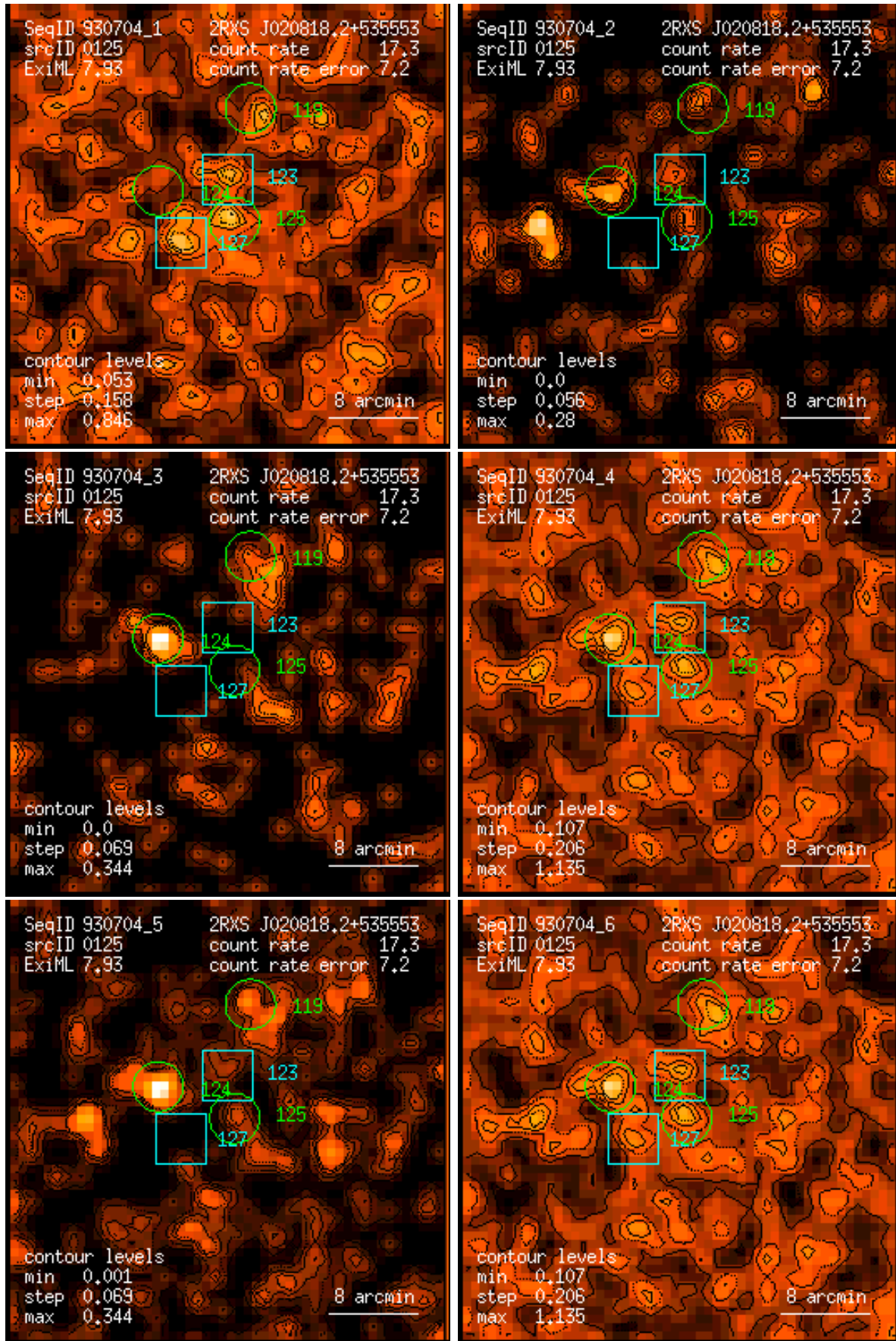
Figure 125: RASS 930704: detection 0125: band rate images, Gaussian filter: (1) PSPC channels 11 – 41, (2) 52 – 90, (3) 91 – 201, (4) 11 – 235, (5) 52 – 201, (6) 11 – 201. Broad band rates in counts/ks. Band rate contour levels in counts/ks/arcmin 2 .
