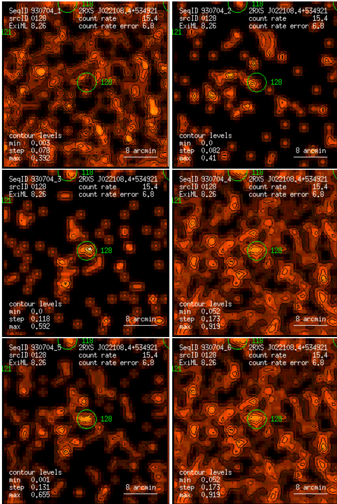
Figure 128: RASS 930704: detection 0128: band rate images, Gaussian filter: (1) PSPC channels 11 – 41, (2) 52 – 90, (3) 91 – 201, (4) 11 – 235, (5) 52 – 201, (6) 11 – 201. Broad band rates in counts/ks. Band rate contour levels in counts/ks/arcmin 2 .
