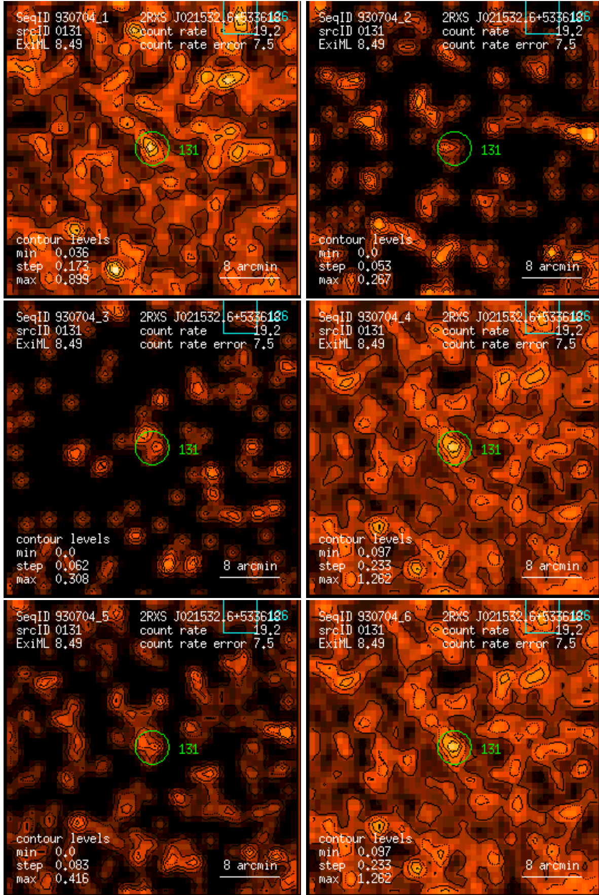
Figure 131: RASS 930704: detection 0131: band rate images, Gaussian filter: (1) PSPC channels 11 – 41, (2) 52 – 90, (3) 91 – 201, (4) 11 – 235, (5) 52 – 201, (6) 11 – 201. Broad band rates in counts/ks. Band rate contour levels in counts/ks/arcmin 2 .
