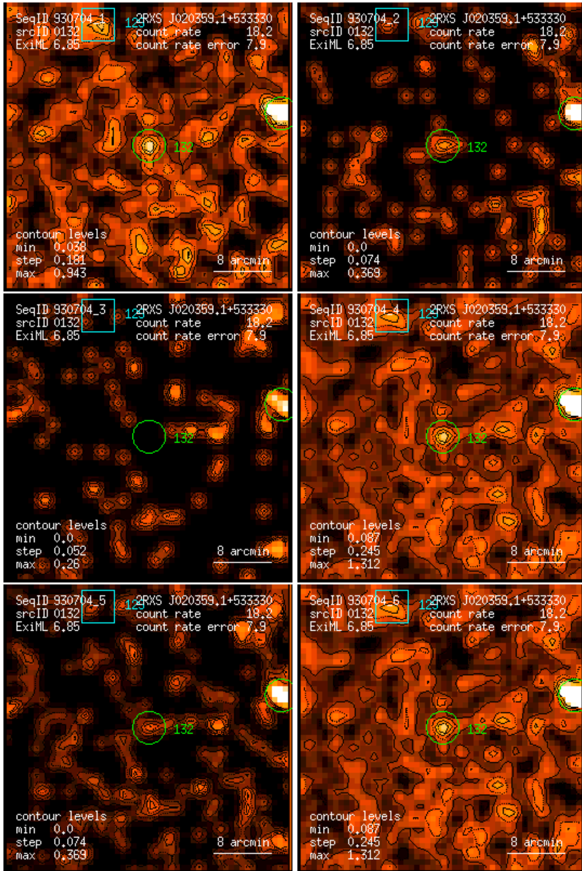
Figure 132: RASS 930704: detection 0132: band rate images, Gaussian filter: (1) PSPC channels 11 – 41, (2) 52 – 90, (3) 91 – 201, (4) 11 – 235, (5) 52 – 201, (6) 11 – 201. Broad band rates in counts/ks. Band rate contour levels in counts/ks/arcmin 2 .
