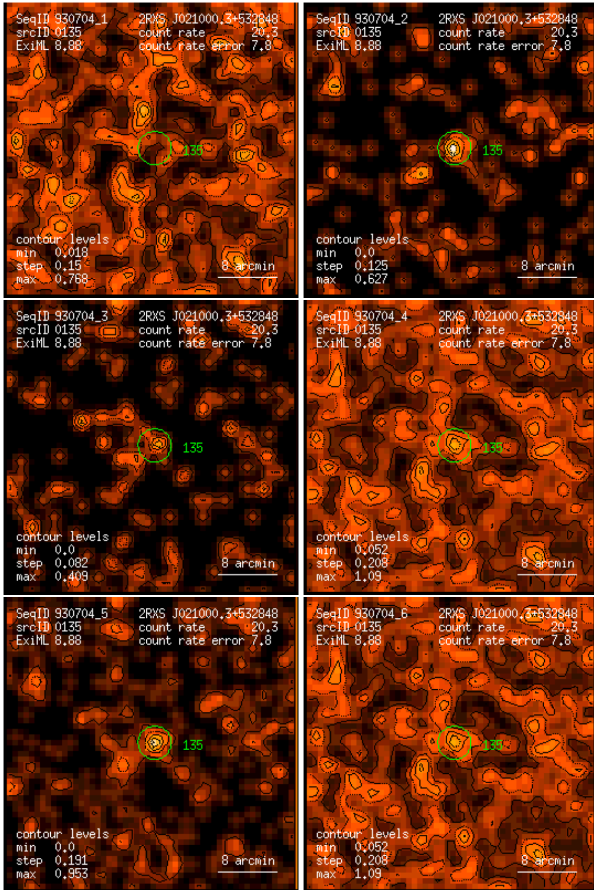
Figure 135: RASS 930704: detection 0135: band rate images, Gaussian filter: (1) PSPC channels 11 – 41, (2) 52 – 90, (3) 91 – 201, (4) 11 – 235, (5) 52 – 201, (6) 11 – 201. Broad band rates in counts/ks. Band rate contour levels in counts/ks/arcmin 2 .
