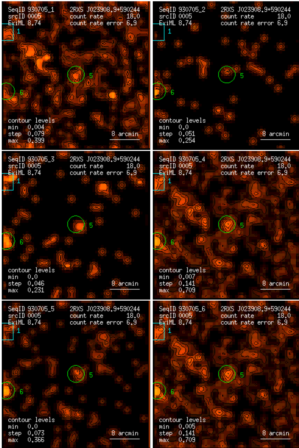
Figure 5: RASS 930705: detection 0005: band rate images, Gaussian filter: (1) PSPC channels 11 – 41, (2) 52 – 90, (3) 91 – 201, (4) 11 – 235, (5) 52 – 201, (6) 11 – 201. Broad band rates in counts/ks. Band rate contour levels in counts/ks/arcmin 2 .
