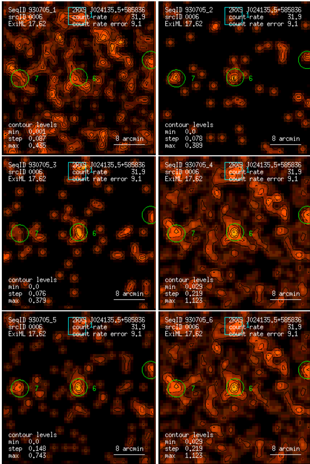
Figure 6: RASS 930705: detection 0006: band rate images, Gaussian filter: (1) PSPC channels 11 – 41, (2) 52 – 90, (3) 91 – 201, (4) 11 – 235, (5) 52 – 201, (6) 11 – 201. Broad band rates in counts/ks. Band rate contour levels in counts/ks/arcmin 2 .
