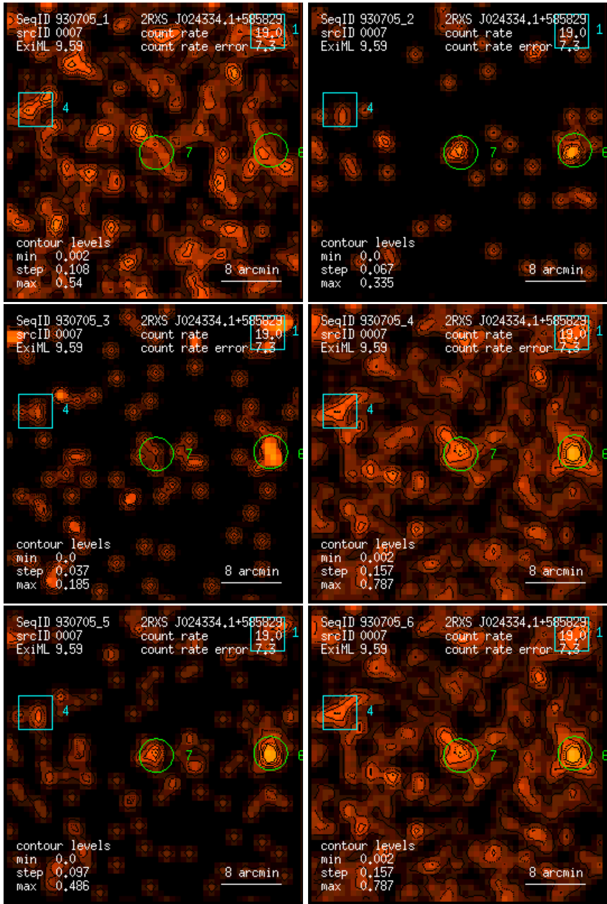
Figure 7: RASS 930705: detection 0007: band rate images, Gaussian filter: (1) PSPC channels 11 – 41, (2) 52 – 90, (3) 91 – 201, (4) 11 – 235, (5) 52 – 201, (6) 11 – 201. Broad band rates in counts/ks. Band rate contour levels in counts/ks/arcmin 2 .
