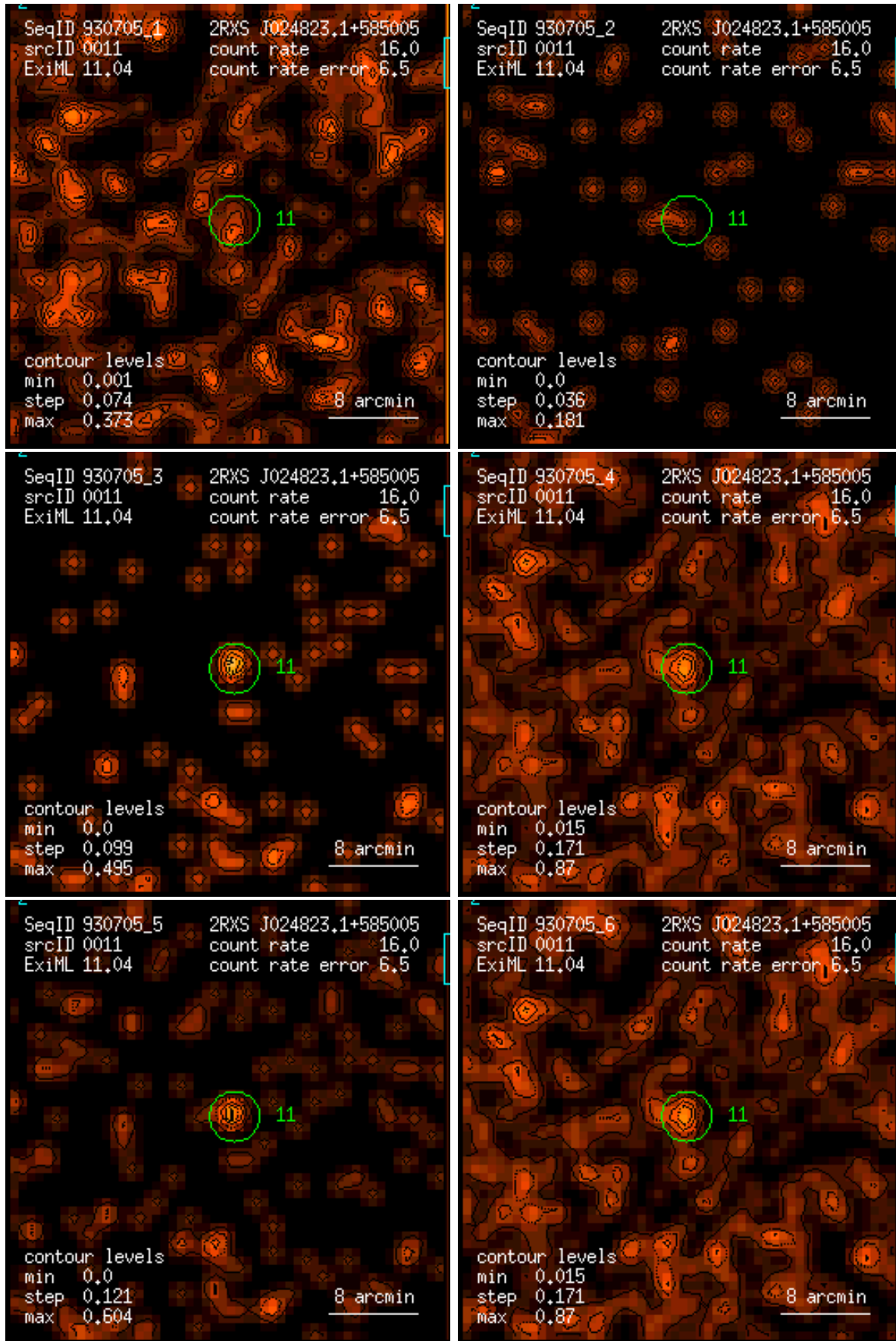
Figure 11: RASS 930705: detection 0011: band rate images, Gaussian filter: (1) PSPC channels 11 – 41, (2) 52 – 90, (3) 91 – 201, (4) 11 – 235, (5) 52 – 201, (6) 11 – 201. Broad band rates in counts/ks. Band rate contour levels in counts/ks/arcmin 2 .
