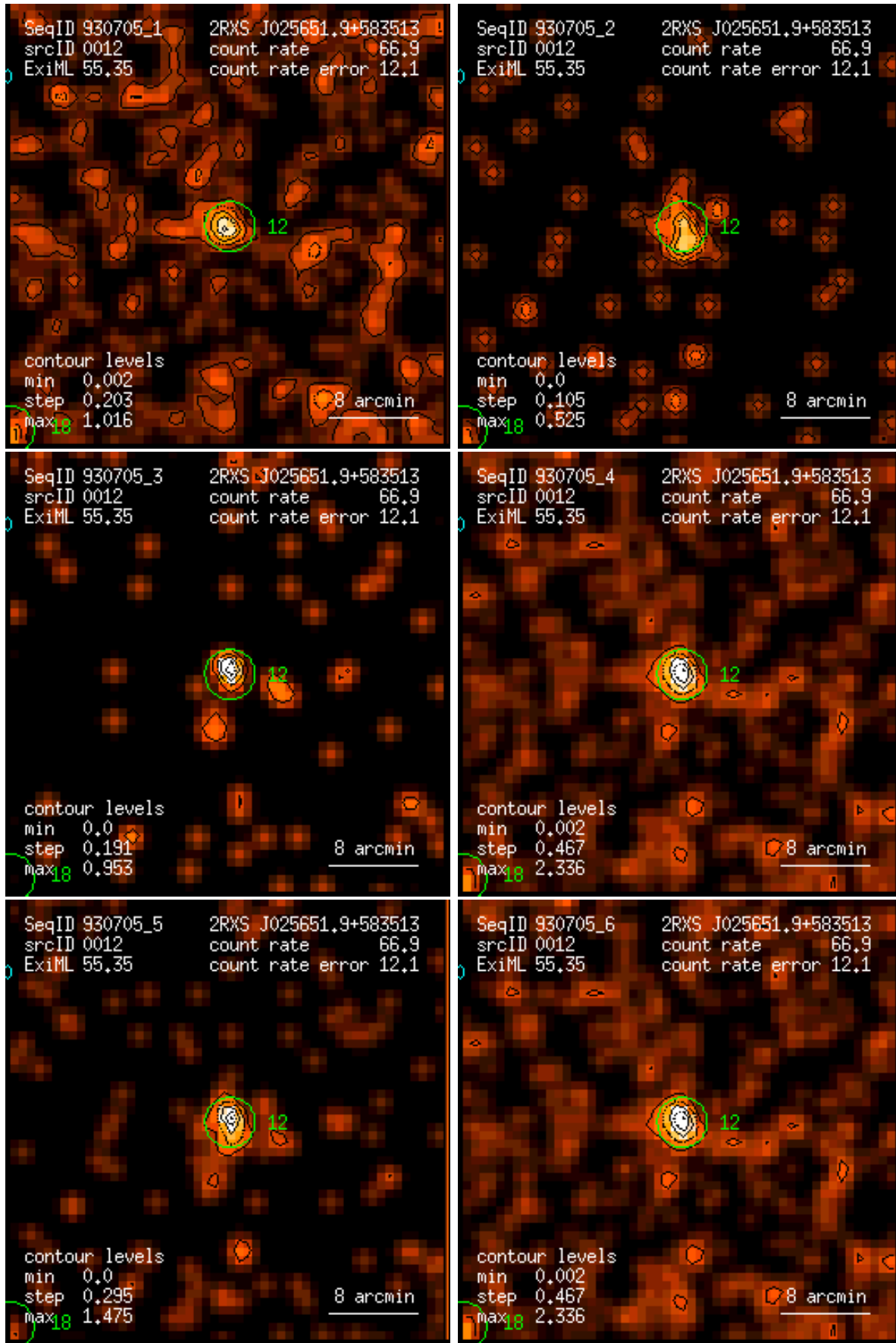
Figure 12: RASS 930705: detection 0012: band rate images, Gaussian filter: (1) PSPC channels 11 – 41, (2) 52 – 90, (3) 91 – 201, (4) 11 – 235, (5) 52 – 201, (6) 11 – 201. Broad band rates in counts/ks. Band rate contour levels in counts/ks/arcmin 2 .
