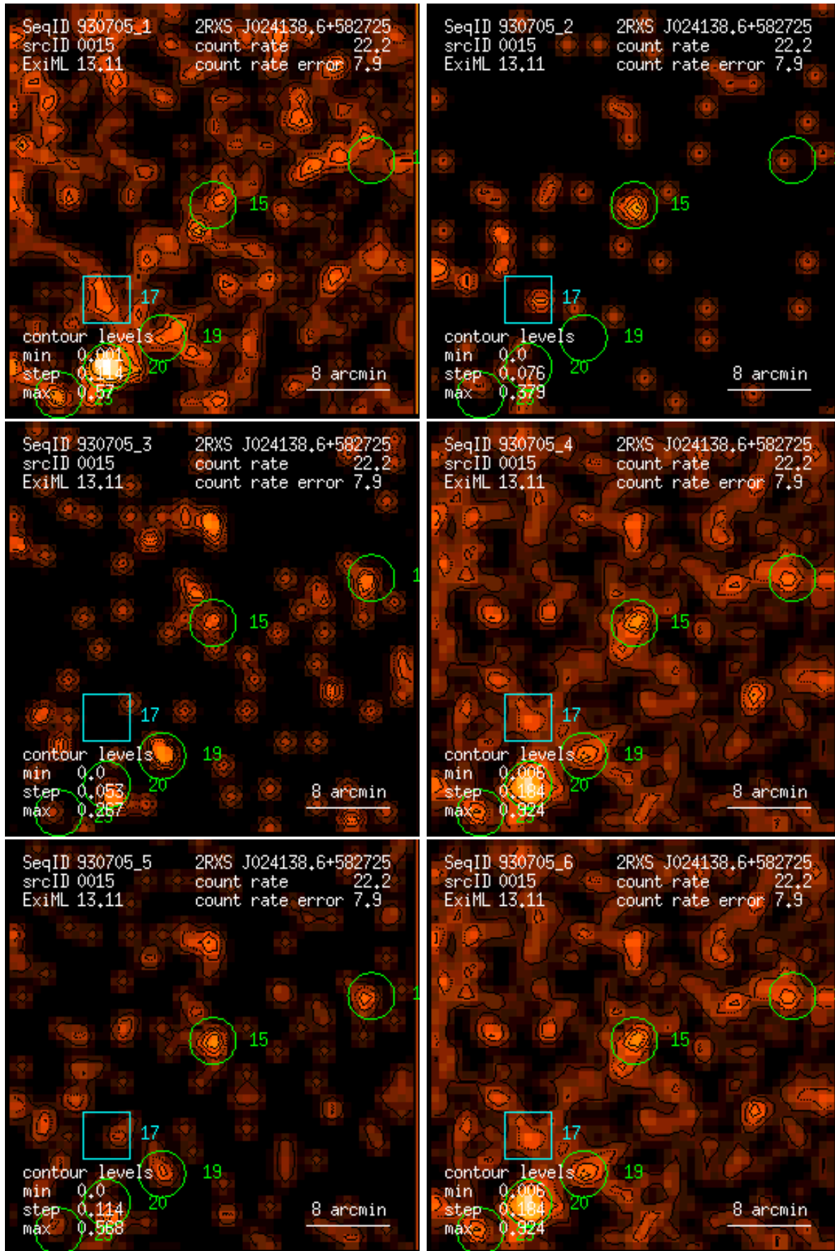
Figure 15: RASS 930705: detection 0015: band rate images, Gaussian filter: (1) PSPC channels 11 – 41, (2) 52 – 90, (3) 91 – 201, (4) 11 – 235, (5) 52 – 201, (6) 11 – 201. Broad band rates in counts/ks. Band rate contour levels in counts/ks/arcmin 2 .
