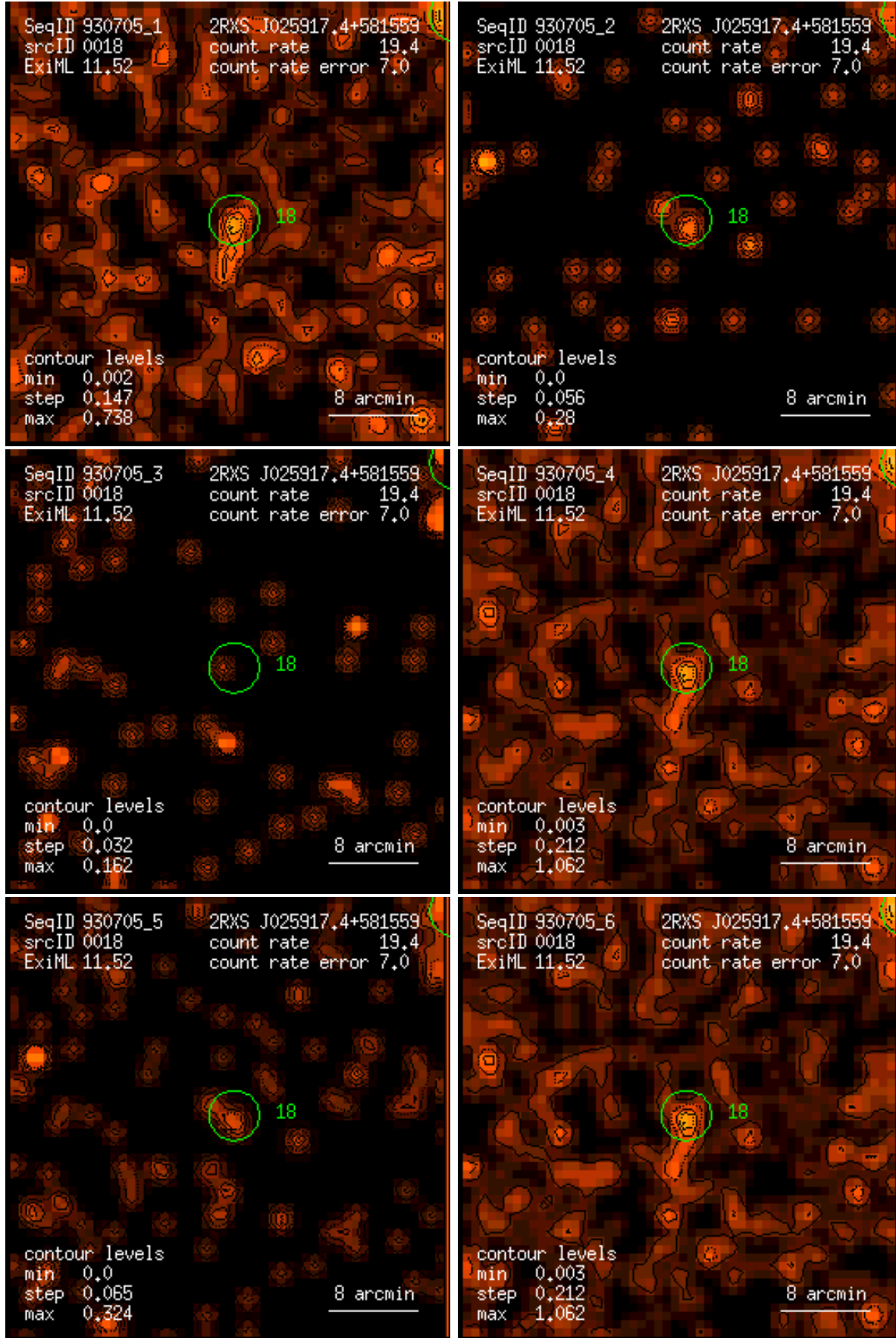
Figure 18: RASS 930705: detection 0018: band rate images, Gaussian filter: (1) PSPC channels 11 – 41, (2) 52 – 90, (3) 91 – 201, (4) 11 – 235, (5) 52 – 201, (6) 11 – 201. Broad band rates in counts/ks. Band rate contour levels in counts/ks/arcmin 2 .
