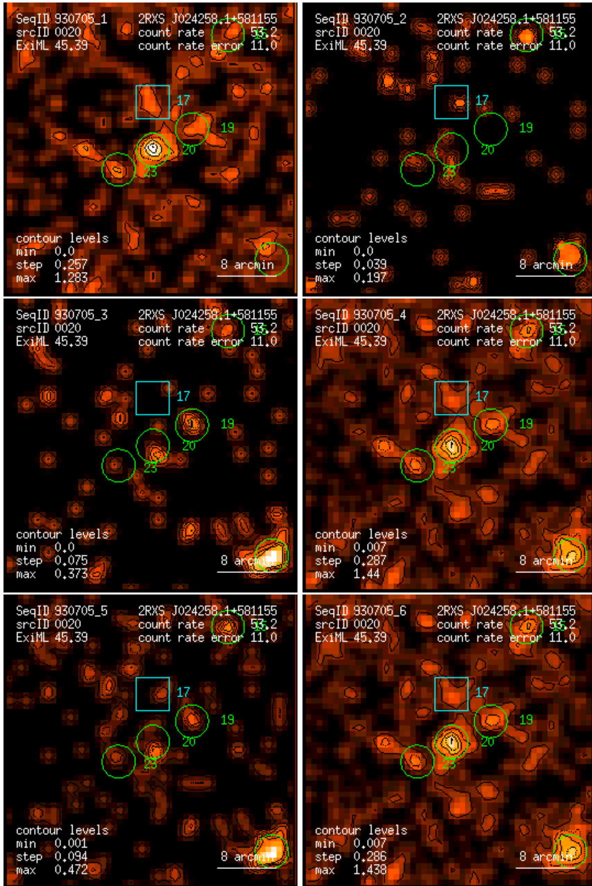
Figure 20: RASS 930705: detection 0020: band rate images, Gaussian filter: (1) PSPC channels 11 – 41, (2) 52 – 90, (3) 91 – 201, (4) 11 – 235, (5) 52 – 201, (6) 11 – 201. Broad band rates in counts/ks. Band rate contour levels in counts/ks/arcmin 2 .
