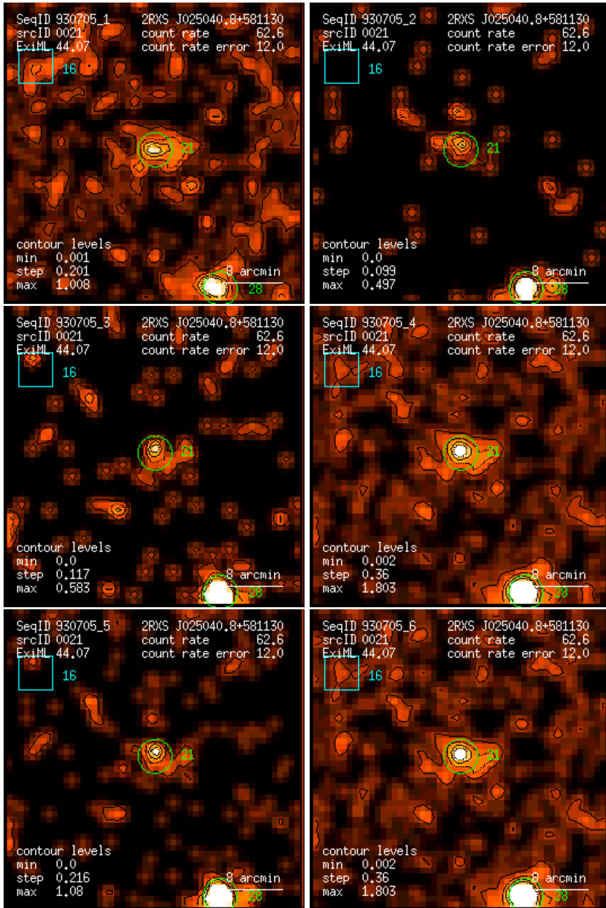
Figure 21: RASS 930705: detection 0021: band rate images, Gaussian filter: (1) PSPC channels 11 – 41, (2) 52 – 90, (3) 91 – 201, (4) 11 – 235, (5) 52 – 201, (6) 11 – 201. Broad band rates in counts/ks. Band rate contour levels in counts/ks/arcmin 2 .
