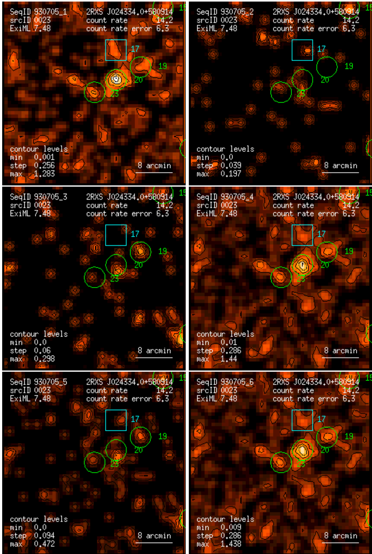
Figure 23: RASS 930705: detection 0023: band rate images, Gaussian filter: (1) PSPC channels 11 – 41, (2) 52 – 90, (3) 91 – 201, (4) 11 – 235, (5) 52 – 201, (6) 11 – 201. Broad band rates in counts/ks. Band rate contour levels in counts/ks/arcmin 2 .
