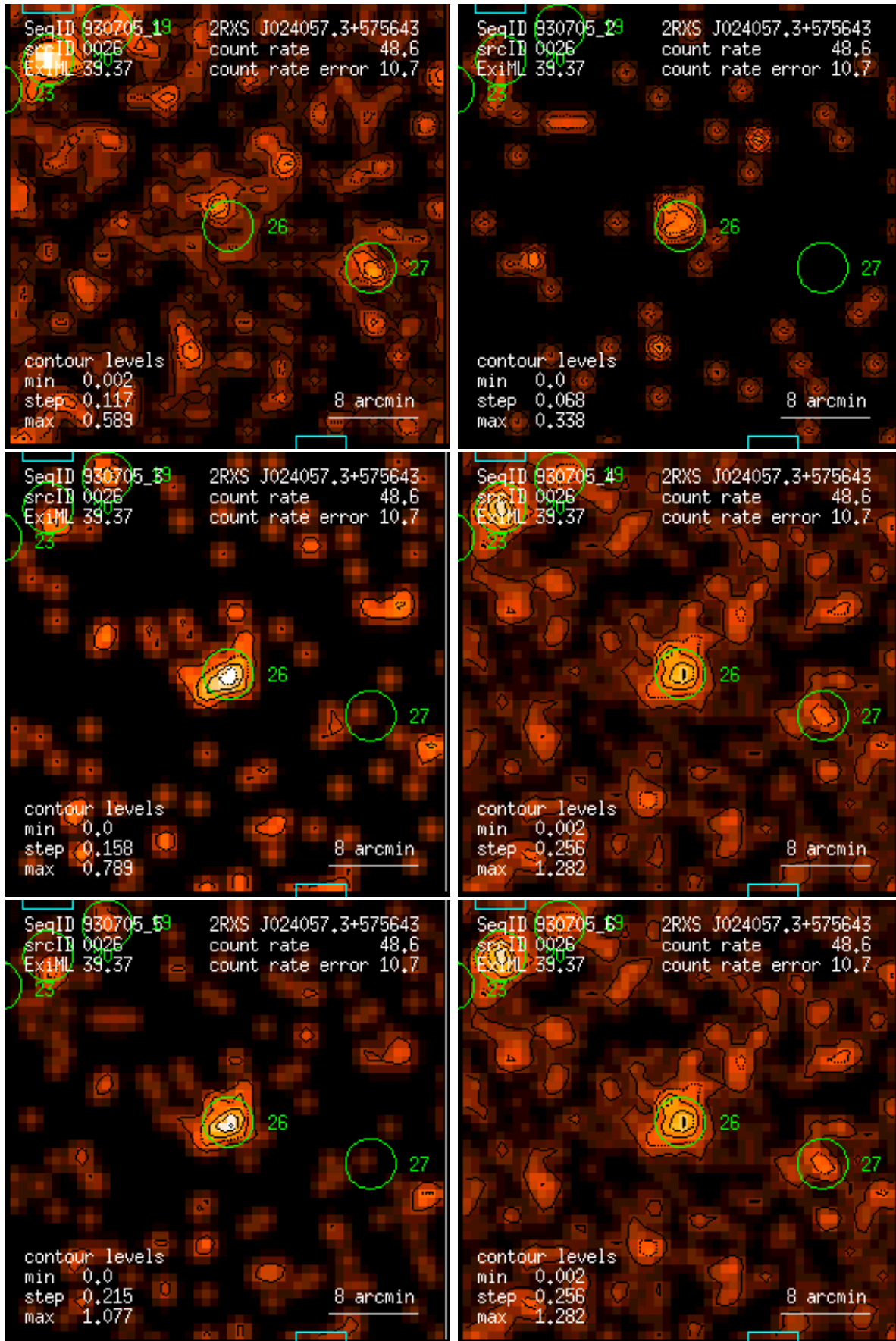
Figure 26: RASS 930705: detection 0026: band rate images, Gaussian filter: (1) PSPC channels 11 – 41, (2) 52 – 90, (3) 91 – 201, (4) 11 – 235, (5) 52 – 201, (6) 11 – 201. Broad band rates in counts/ks. Band rate contour levels in counts/ks/arcmin 2 .
