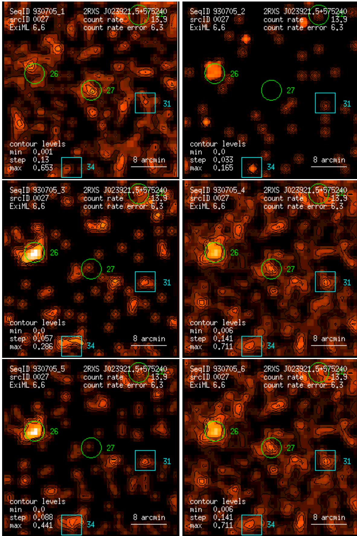
Figure 27: RASS 930705: detection 0027: band rate images, Gaussian filter: (1) PSPC channels 11 – 41, (2) 52 – 90, (3) 91 – 201, (4) 11 – 235, (5) 52 – 201, (6) 11 – 201. Broad band rates in counts/ks. Band rate contour levels in counts/ks/arcmin 2 .
