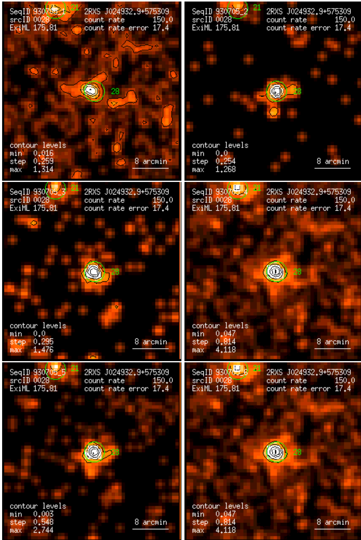
Figure 28: RASS 930705: detection 0028: band rate images, Gaussian filter: (1) PSPC channels 11 – 41, (2) 52 – 90, (3) 91 – 201, (4) 11 – 235, (5) 52 – 201, (6) 11 – 201. Broad band rates in counts/ks. Band rate contour levels in counts/ks/arcmin 2 .
