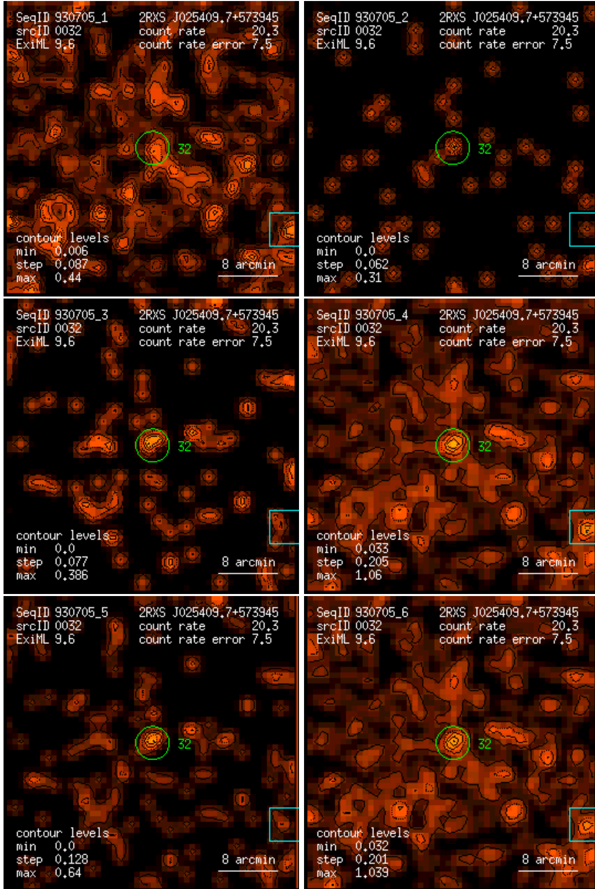
Figure 32: RASS 930705: detection 0032: band rate images, Gaussian filter: (1) PSPC channels 11 – 41, (2) 52 – 90, (3) 91 – 201, (4) 11 – 235, (5) 52 – 201, (6) 11 – 201. Broad band rates in counts/ks. Band rate contour levels in counts/ks/arcmin 2 .
