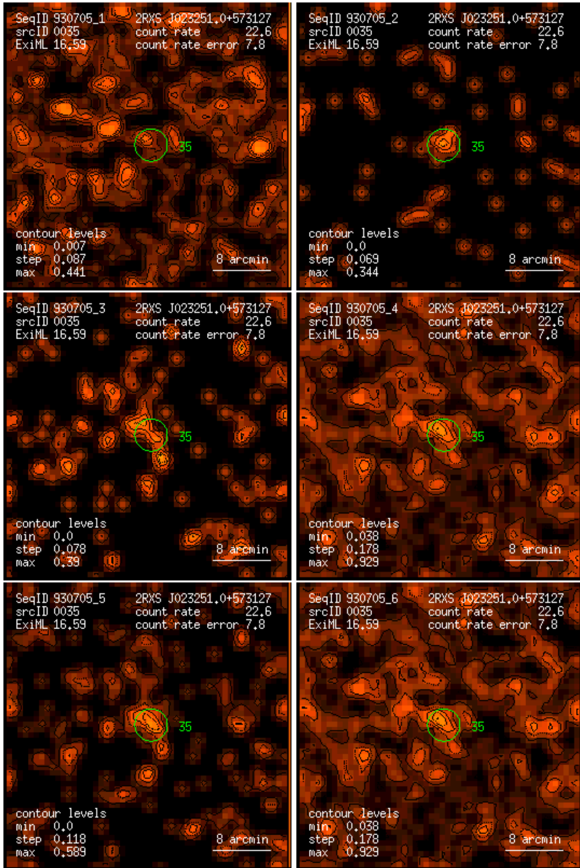
Figure 35: RASS 930705: detection 0035: band rate images, Gaussian filter: (1) PSPC channels 11 – 41, (2) 52 – 90, (3) 91 – 201, (4) 11 – 235, (5) 52 – 201, (6) 11 – 201. Broad band rates in counts/ks. Band rate contour levels in counts/ks/arcmin 2 .
