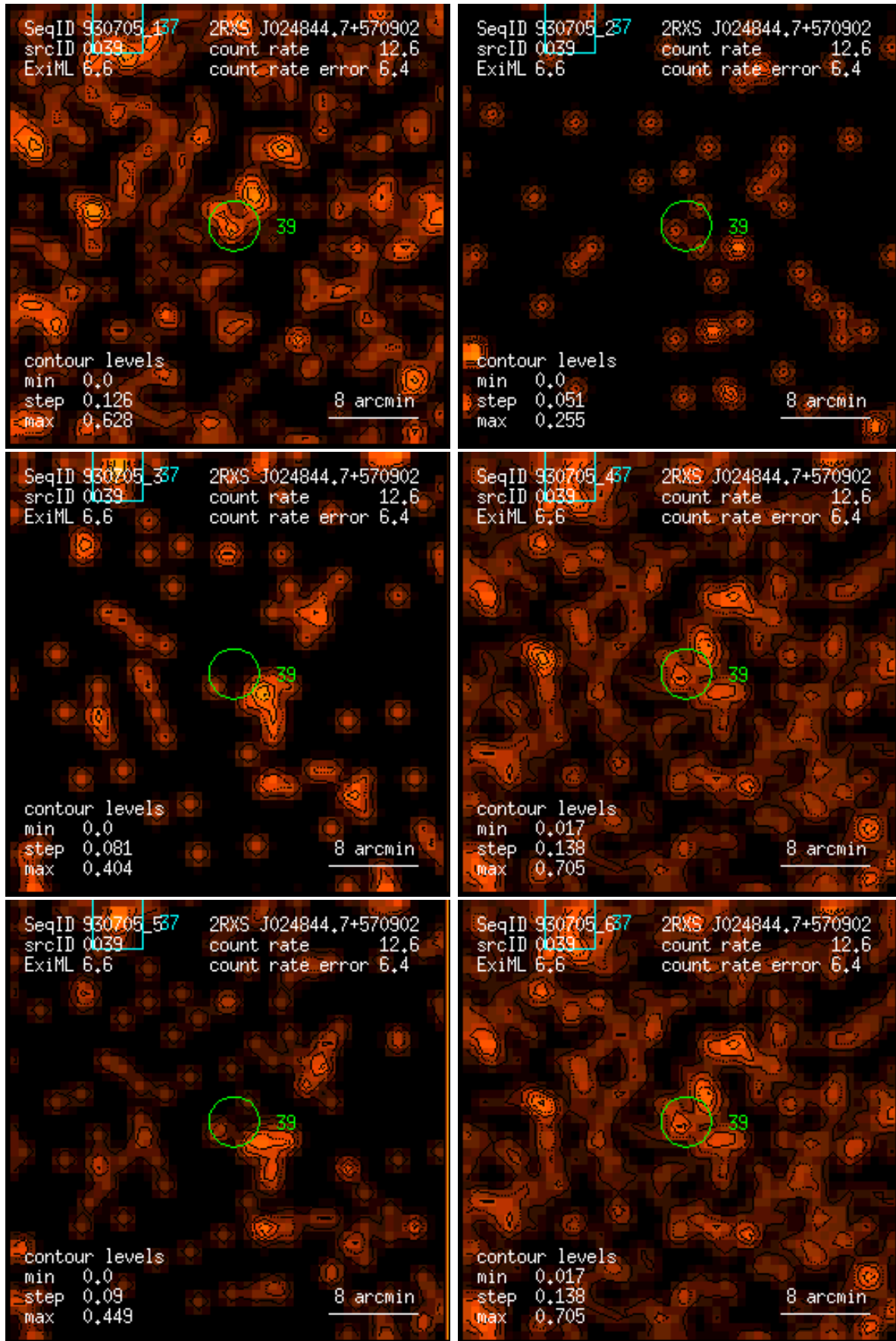
Figure 39: RASS 930705: detection 0039: band rate images, Gaussian filter: (1) PSPC channels 11 – 41, (2) 52 – 90, (3) 91 – 201, (4) 11 – 235, (5) 52 – 201, (6) 11 – 201. Broad band rates in counts/ks. Band rate contour levels in counts/ks/arcmin 2 .
