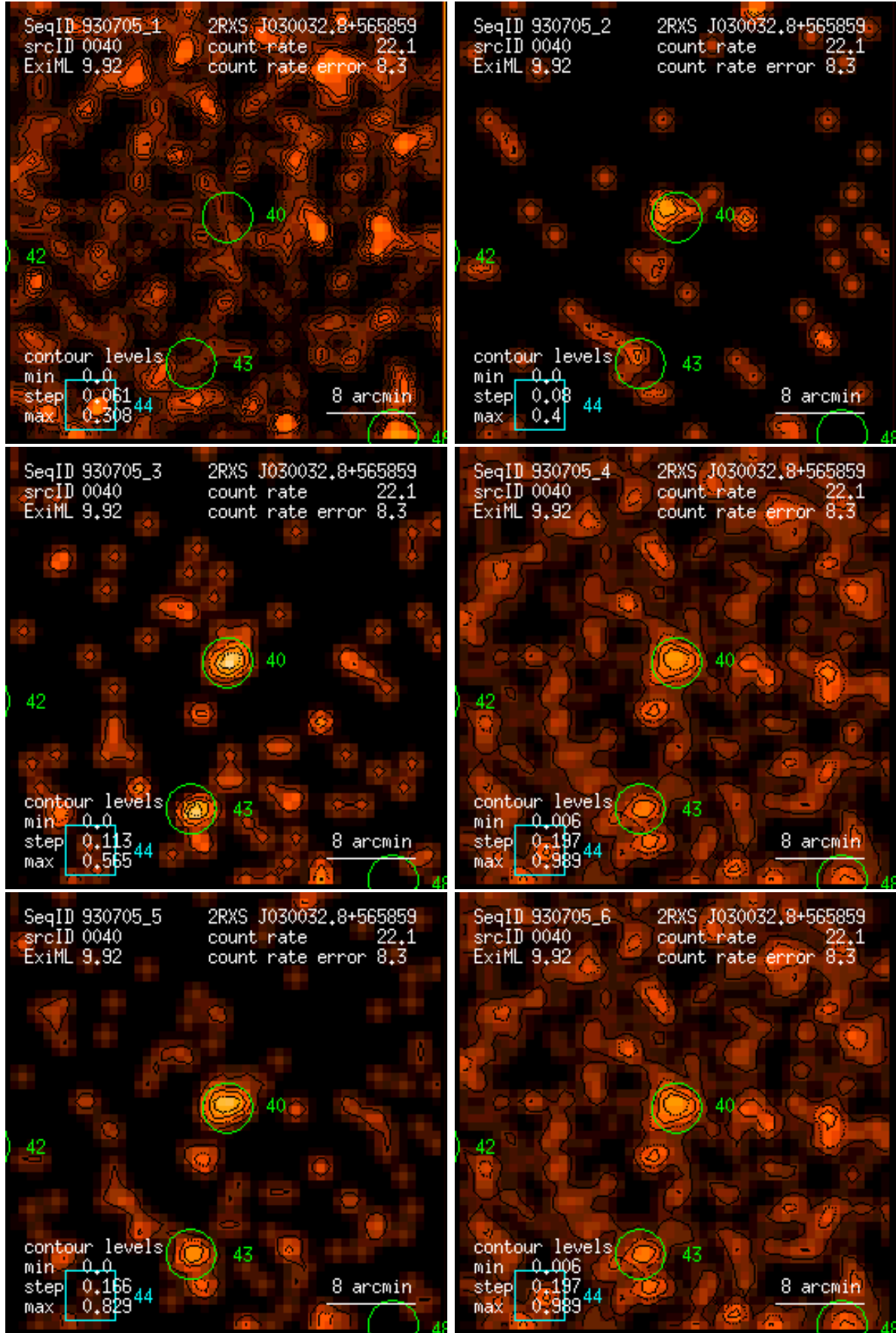
Figure 40: RASS 930705: detection 0040: band rate images, Gaussian filter: (1) PSPC channels 11 – 41, (2) 52 – 90, (3) 91 – 201, (4) 11 – 235, (5) 52 – 201, (6) 11 – 201. Broad band rates in counts/ks. Band rate contour levels in counts/ks/arcmin 2 .
