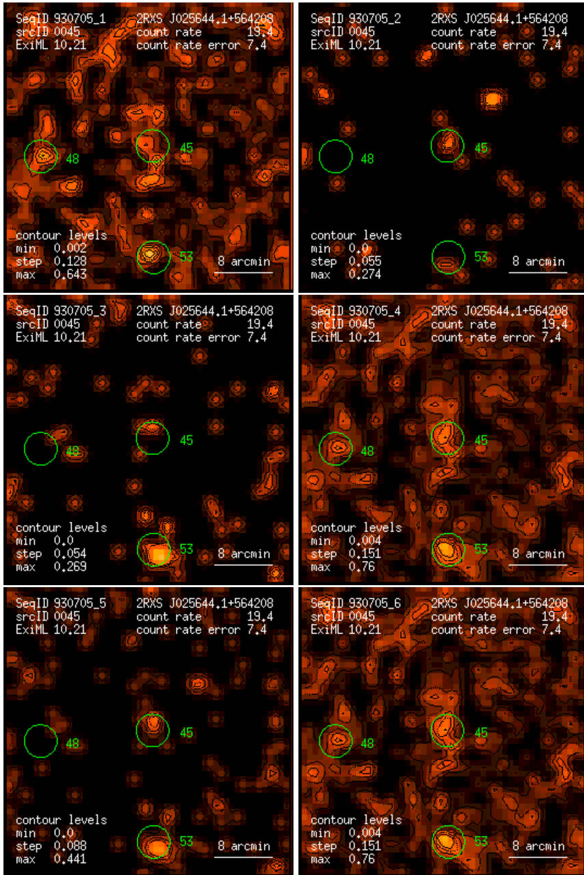
Figure 45: RASS 930705: detection 0045: band rate images, Gaussian filter: (1) PSPC channels 11 – 41, (2) 52 – 90, (3) 91 – 201, (4) 11 – 235, (5) 52 – 201, (6) 11 – 201. Broad band rates in counts/ks. Band rate contour levels in counts/ks/arcmin 2 .
