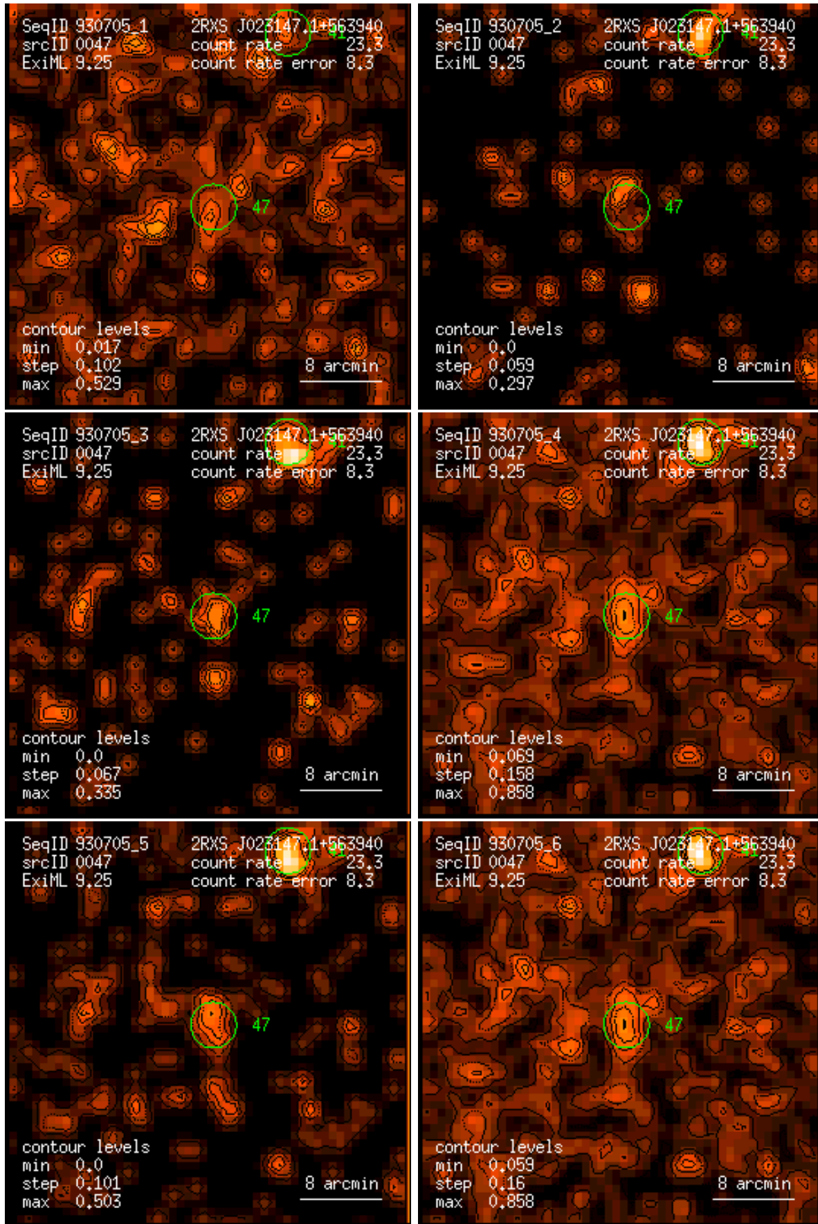
Figure 47: RASS 930705: detection 0047: band rate images, Gaussian filter: (1) PSPC channels 11 – 41, (2) 52 – 90, (3) 91 – 201, (4) 11 – 235, (5) 52 – 201, (6) 11 – 201. Broad band rates in counts/ks. Band rate contour levels in counts/ks/arcmin 2 .
