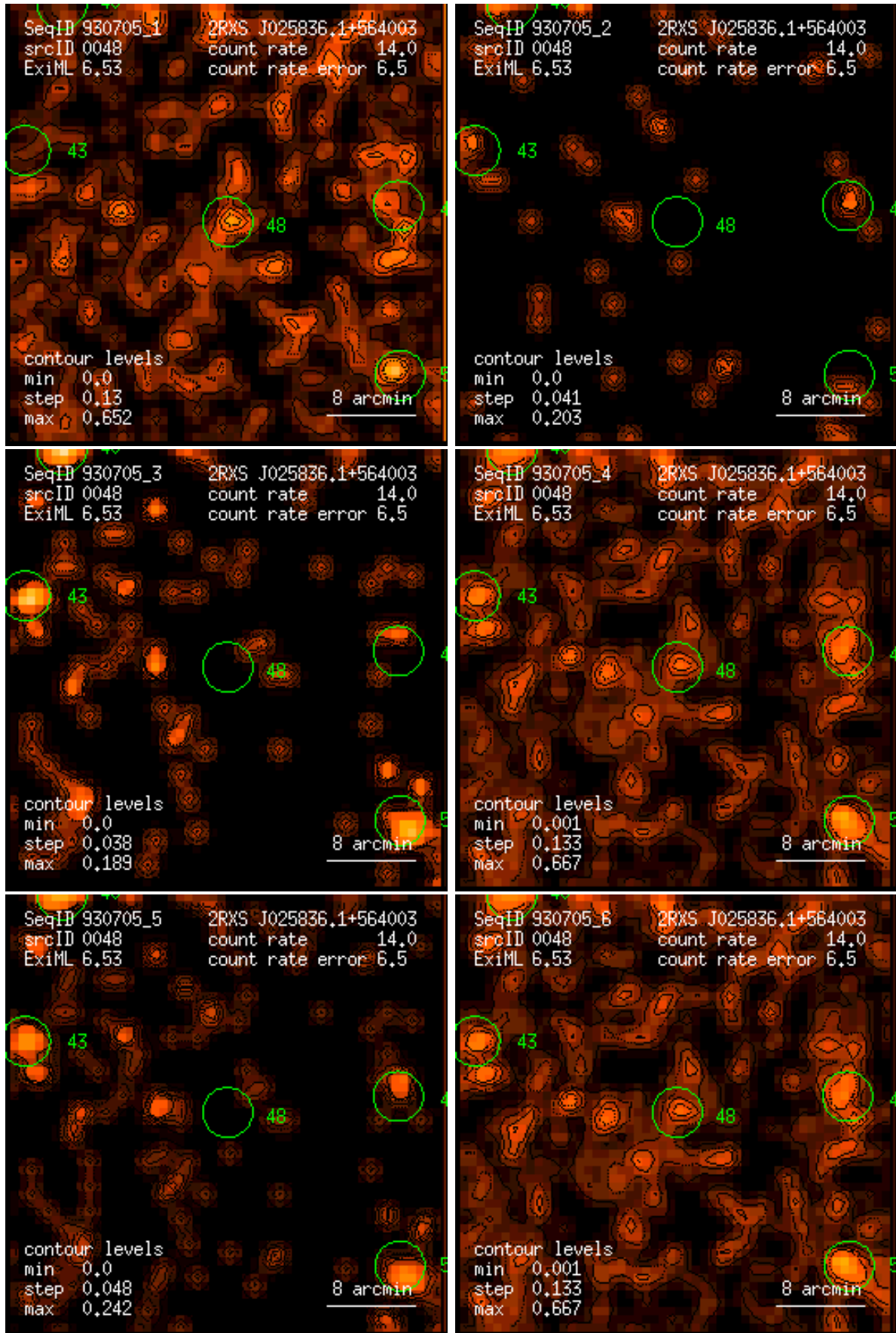
Figure 48: RASS 930705: detection 0048: band rate images, Gaussian filter: (1) PSPC channels 11 – 41, (2) 52 – 90, (3) 91 – 201, (4) 11 – 235, (5) 52 – 201, (6) 11 – 201. Broad band rates in counts/ks. Band rate contour levels in counts/ks/arcmin 2 .
