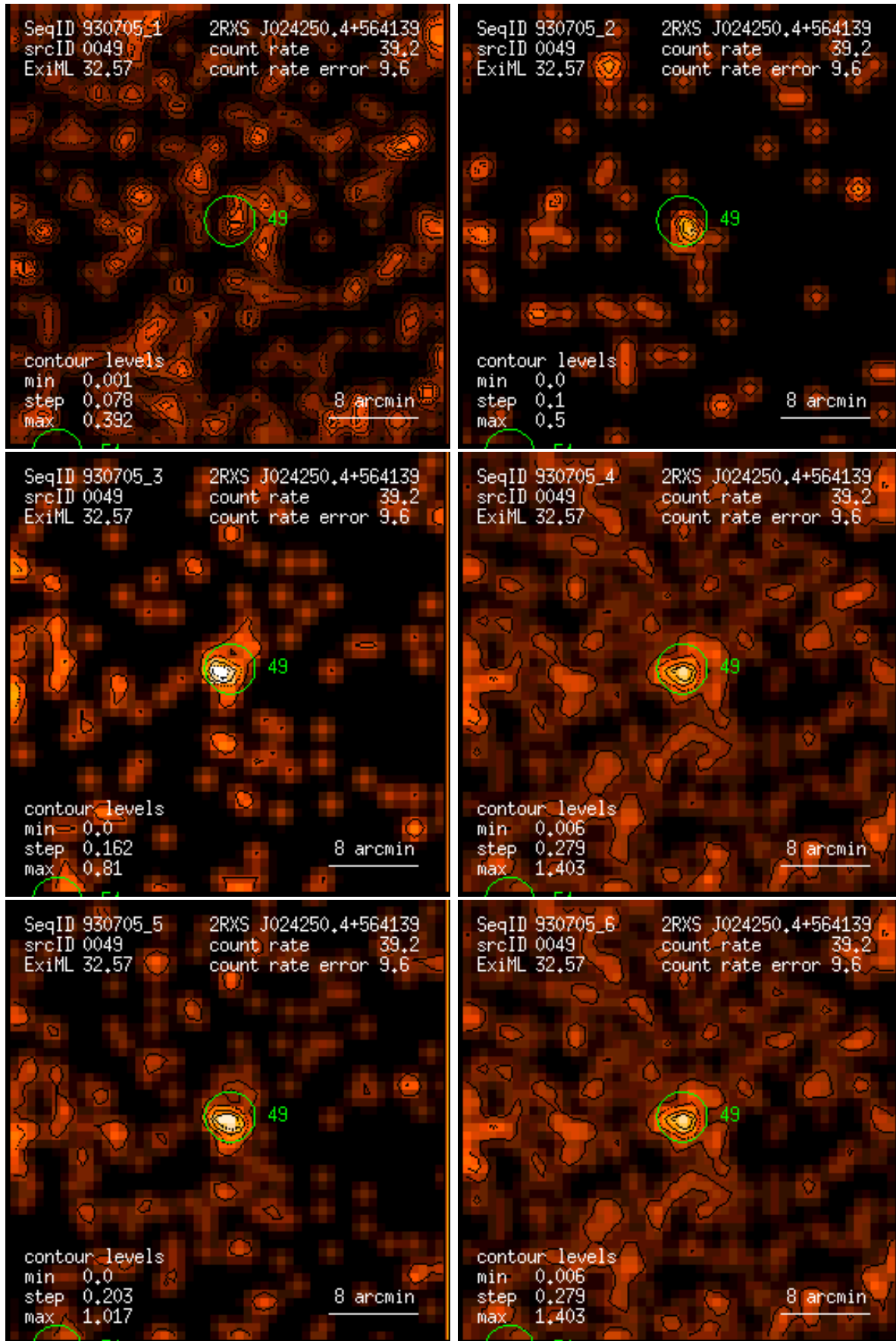
Figure 49: RASS 930705: detection 0049: band rate images, Gaussian filter: (1) PSPC channels 11 – 41, (2) 52 – 90, (3) 91 – 201, (4) 11 – 235, (5) 52 – 201, (6) 11 – 201. Broad band rates in counts/ks. Band rate contour levels in counts/ks/arcmin 2 .
