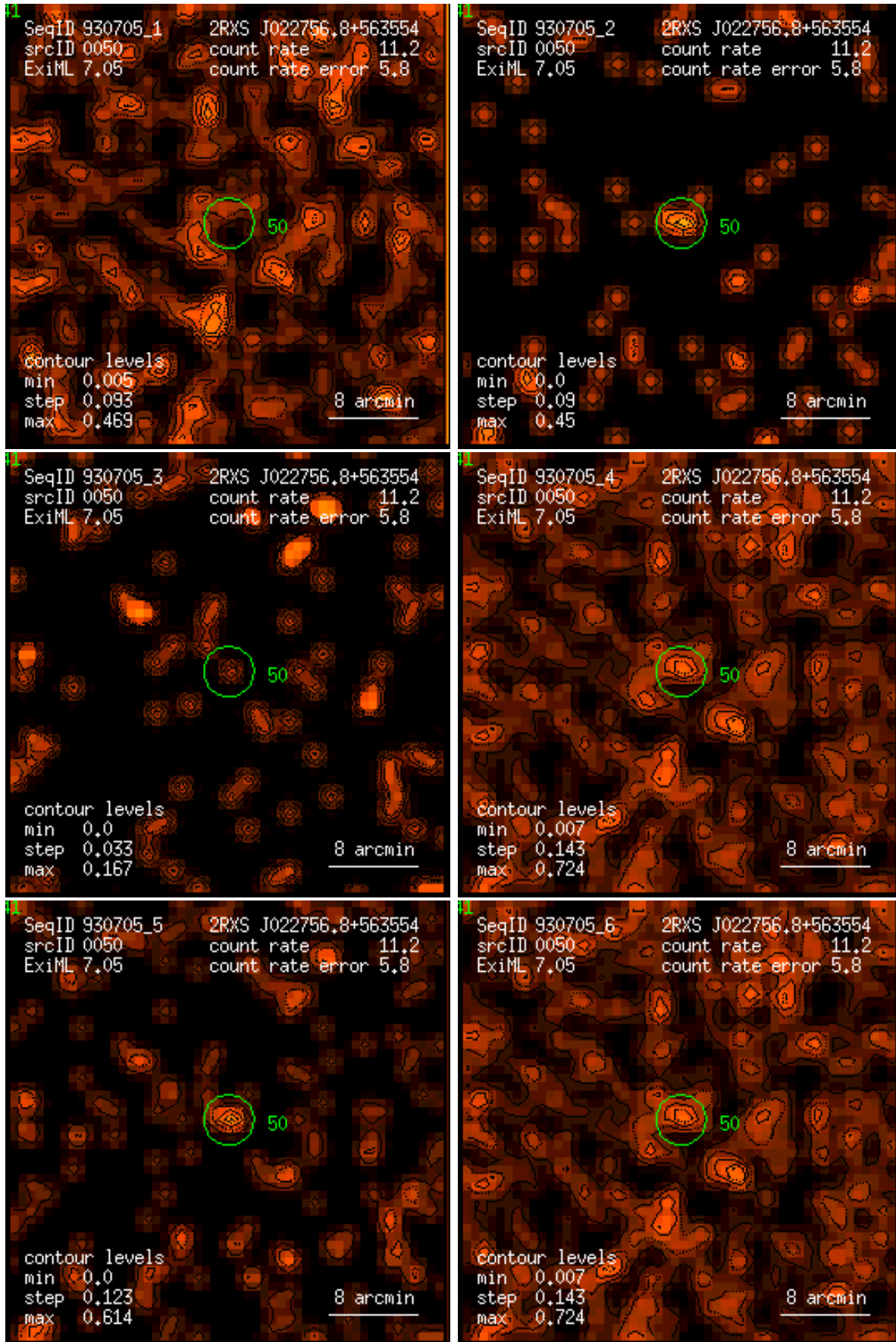
Figure 50: RASS 930705: detection 0050: band rate images, Gaussian filter: (1) PSPC channels 11 – 41, (2) 52 – 90, (3) 91 – 201, (4) 11 – 235, (5) 52 – 201, (6) 11 – 201. Broad band rates in counts/ks. Band rate contour levels in counts/ks/arcmin 2 .
