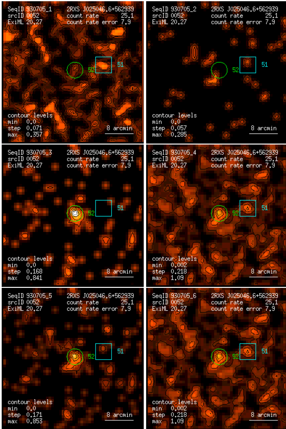
Figure 52: RASS 930705: detection 0052: band rate images, Gaussian filter: (1) PSPC channels 11 – 41, (2) 52 – 90, (3) 91 – 201, (4) 11 – 235, (5) 52 – 201, (6) 11 – 201. Broad band rates in counts/ks. Band rate contour levels in counts/ks/arcmin 2 .
