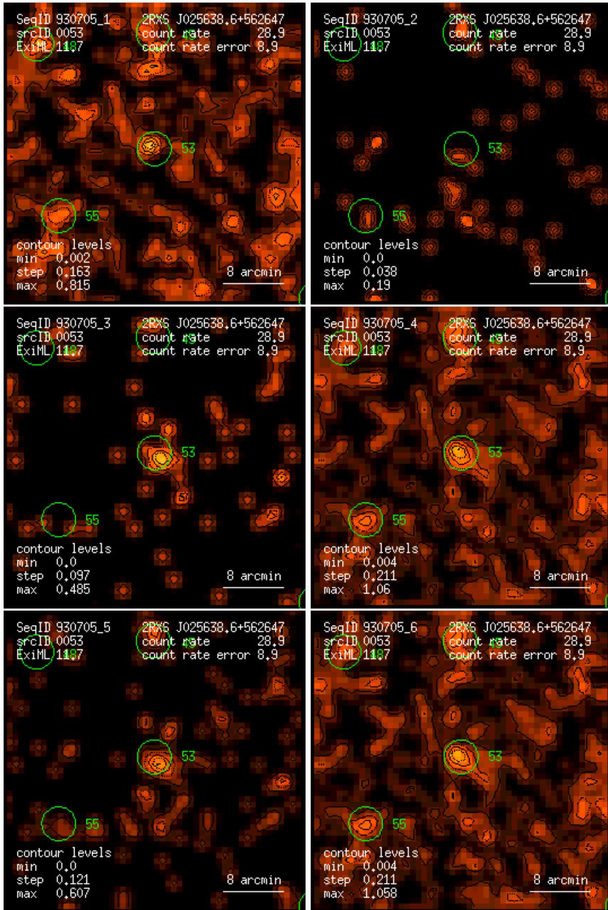
Figure 53: RASS 930705: detection 0053: band rate images, Gaussian filter: (1) PSPC channels 11 – 41, (2) 52 – 90, (3) 91 – 201, (4) 11 – 235, (5) 52 – 201, (6) 11 – 201. Broad band rates in counts/ks. Band rate contour levels in counts/ks/arcmin 2 .
