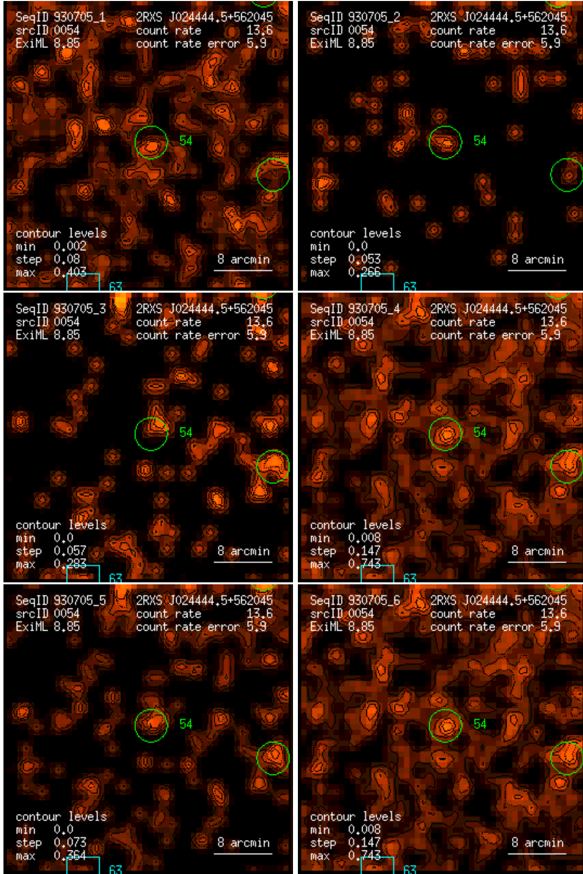
Figure 54: RASS 930705: detection 0054: band rate images, Gaussian filter: (1) PSPC channels 11 – 41, (2) 52 – 90, (3) 91 – 201, (4) 11 – 235, (5) 52 – 201, (6) 11 – 201. Broad band rates in counts/ks. Band rate contour levels in counts/ks/arcmin 2 .
