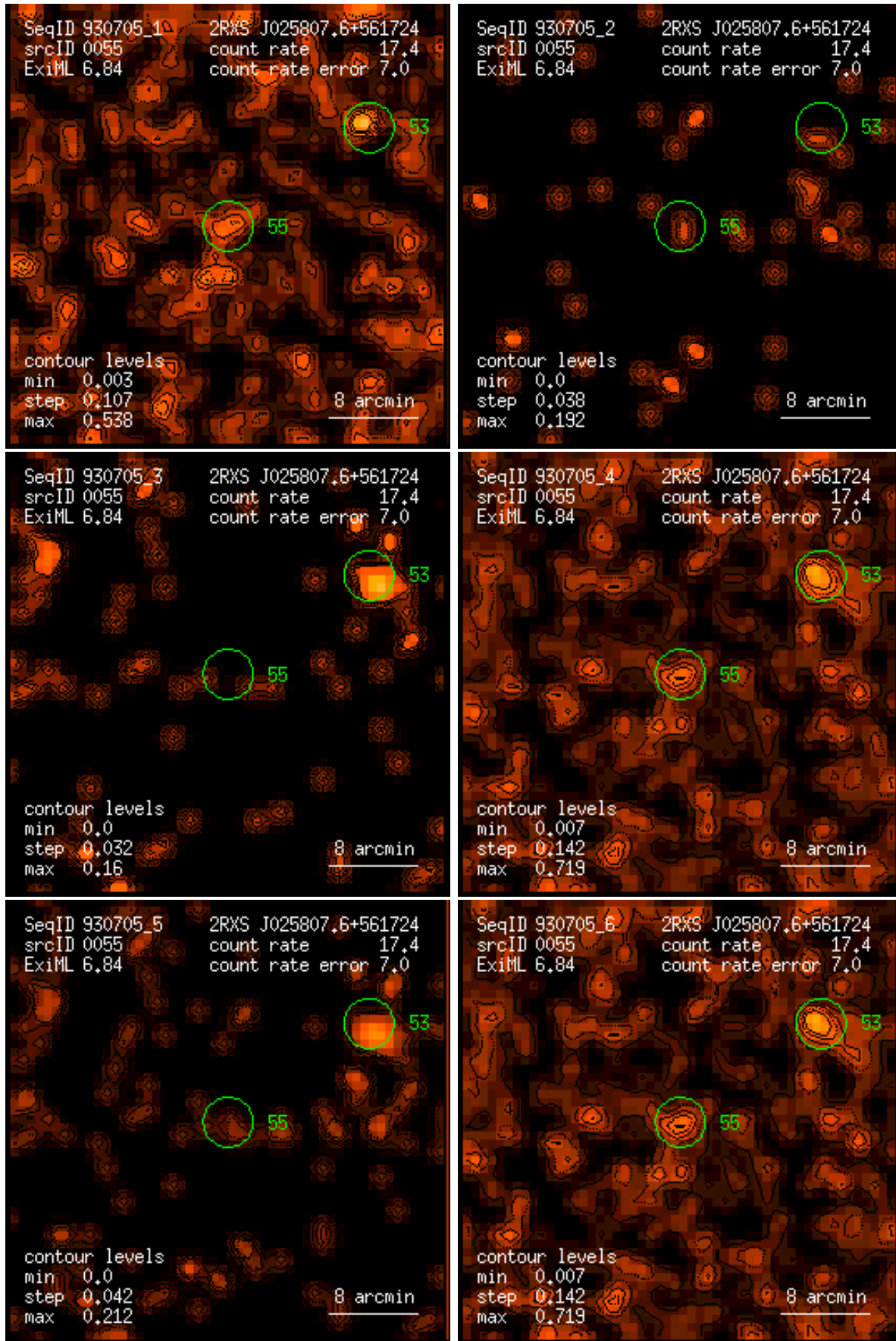
Figure 55: RASS 930705: detection 0055: band rate images, Gaussian filter: (1) PSPC channels 11 – 41, (2) 52 – 90, (3) 91 – 201, (4) 11 – 235, (5) 52 – 201, (6) 11 – 201. Broad band rates in counts/ks. Band rate contour levels in counts/ks/arcmin 2 .
