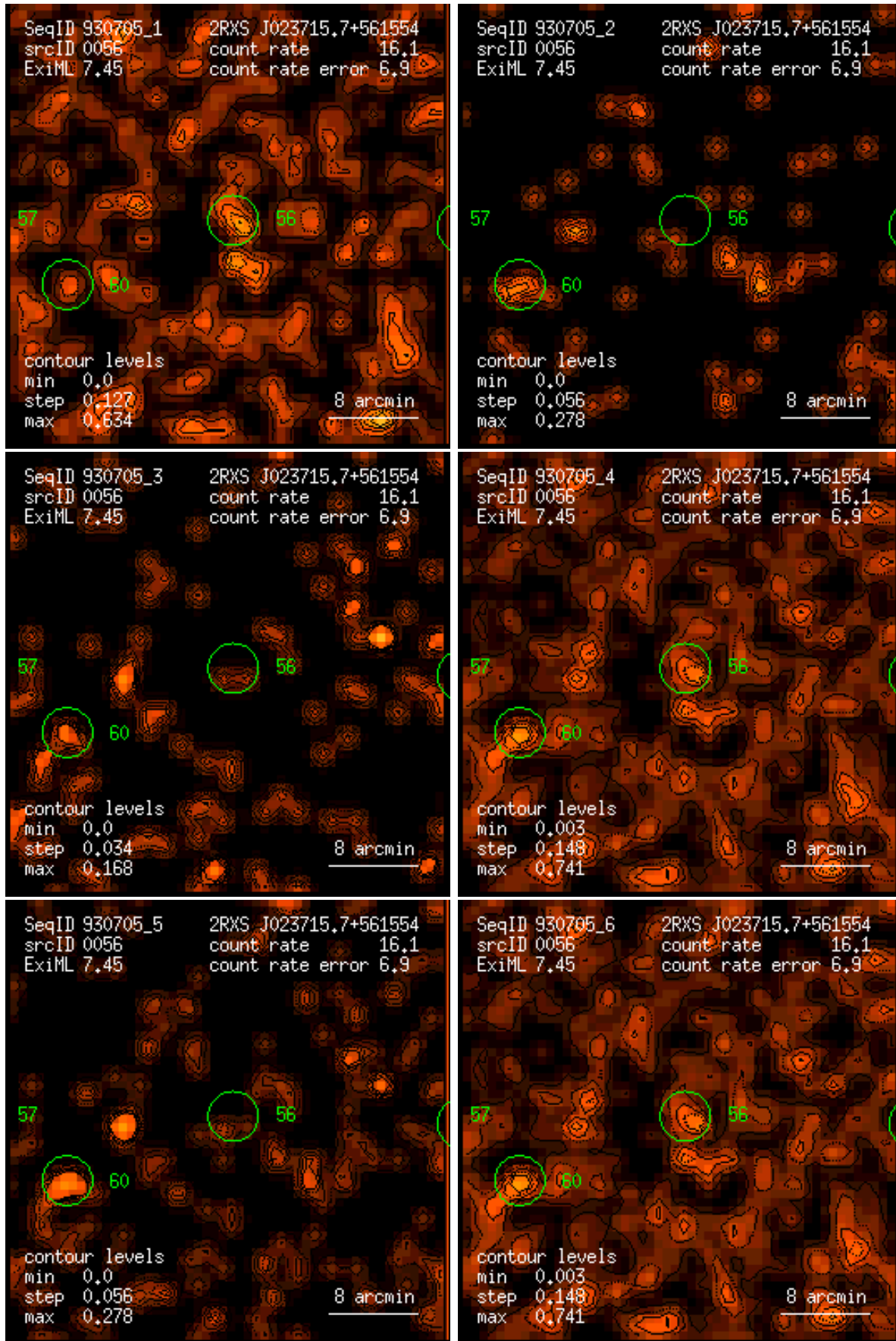
Figure 56: RASS 930705: detection 0056: band rate images, Gaussian filter: (1) PSPC channels 11 – 41, (2) 52 – 90, (3) 91 – 201, (4) 11 – 235, (5) 52 – 201, (6) 11 – 201. Broad band rates in counts/ks. Band rate contour levels in counts/ks/arcmin 2 .
