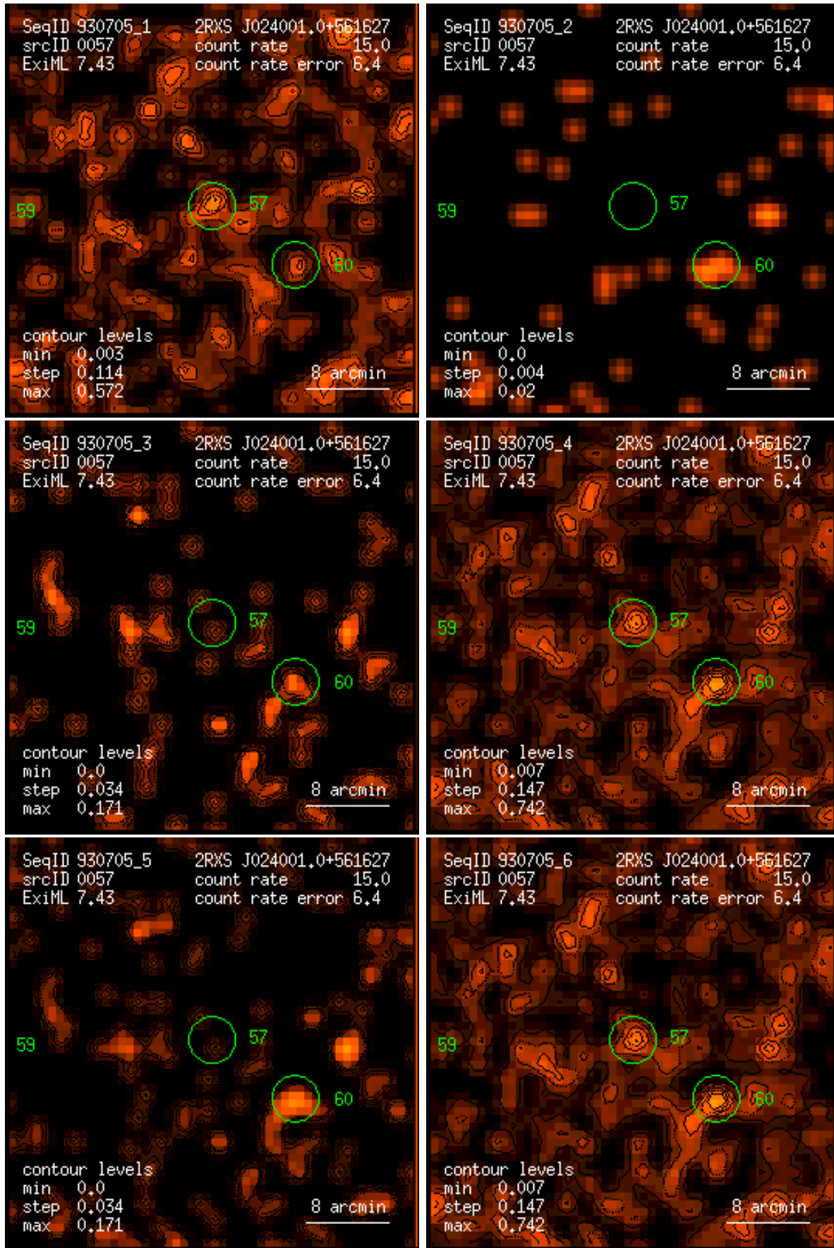
Figure 57: RASS 930705: detection 0057: band rate images, Gaussian filter: (1) PSPC channels 11 – 41, (2) 52 – 90, (3) 91 – 201, (4) 11 – 235, (5) 52 – 201, (6) 11 – 201. Broad band rates in counts/ks. Band rate contour levels in counts/ks/arcmin 2 .
