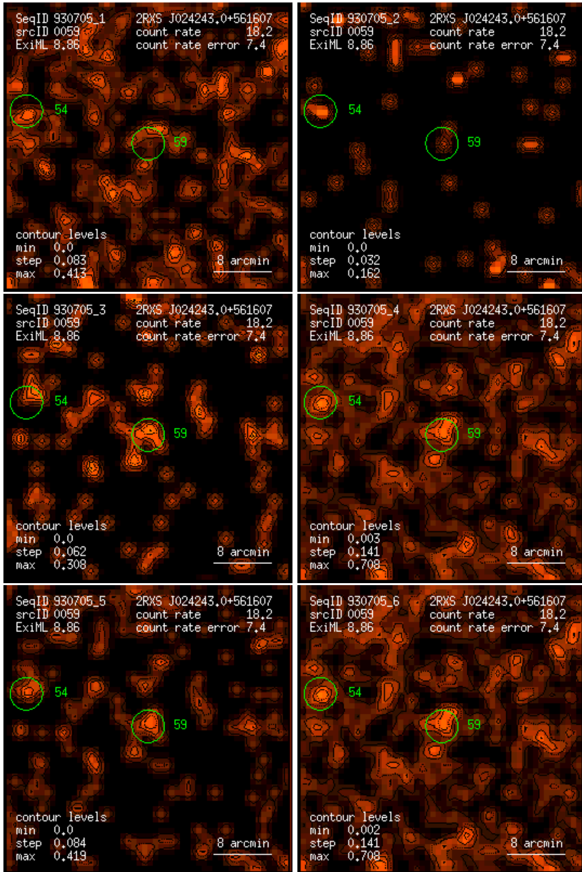
Figure 59: RASS 930705: detection 0059: band rate images, Gaussian filter: (1) PSPC channels 11 – 41, (2) 52 – 90, (3) 91 – 201, (4) 11 – 235, (5) 52 – 201, (6) 11 – 201. Broad band rates in counts/ks. Band rate contour levels in counts/ks/arcmin 2 .
