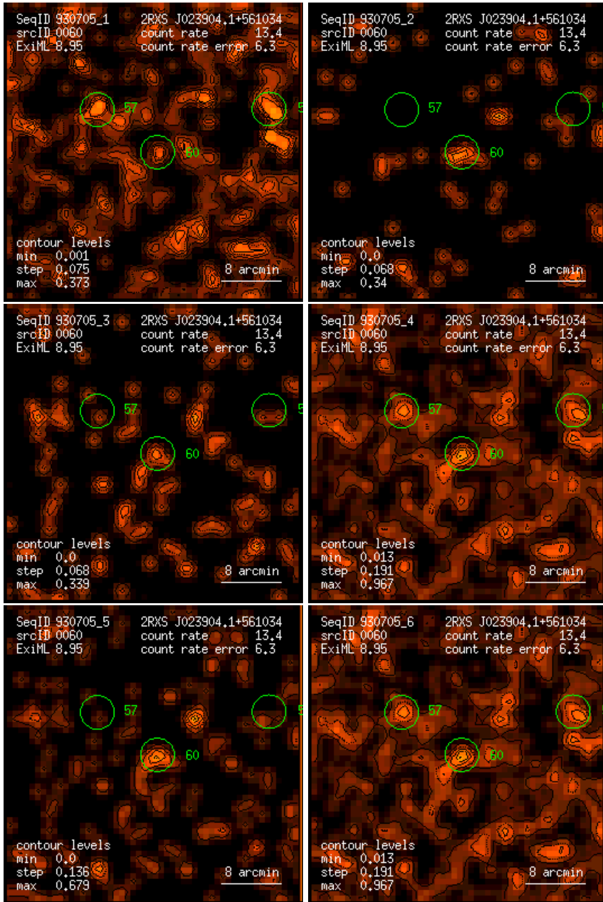
Figure 60: RASS 930705: detection 0060: band rate images, Gaussian filter: (1) PSPC channels 11 – 41, (2) 52 – 90, (3) 91 – 201, (4) 11 – 235, (5) 52 – 201, (6) 11 – 201. Broad band rates in counts/ks. Band rate contour levels in counts/ks/arcmin 2 .
