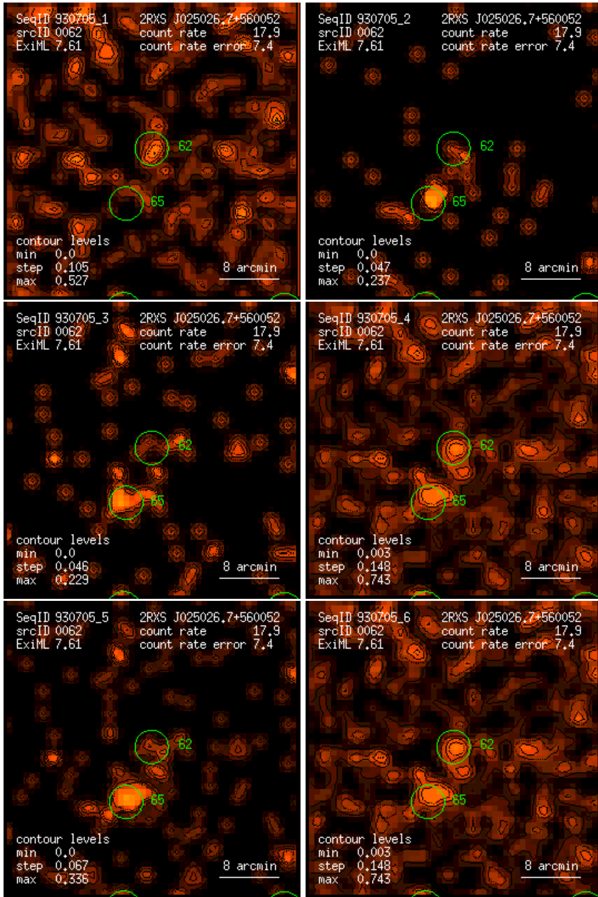
Figure 62: RASS 930705: detection 0062: band rate images, Gaussian filter: (1) PSPC channels 11 – 41, (2) 52 – 90, (3) 91 – 201, (4) 11 – 235, (5) 52 – 201, (6) 11 – 201. Broad band rates in counts/ks. Band rate contour levels in counts/ks/arcmin 2 .
