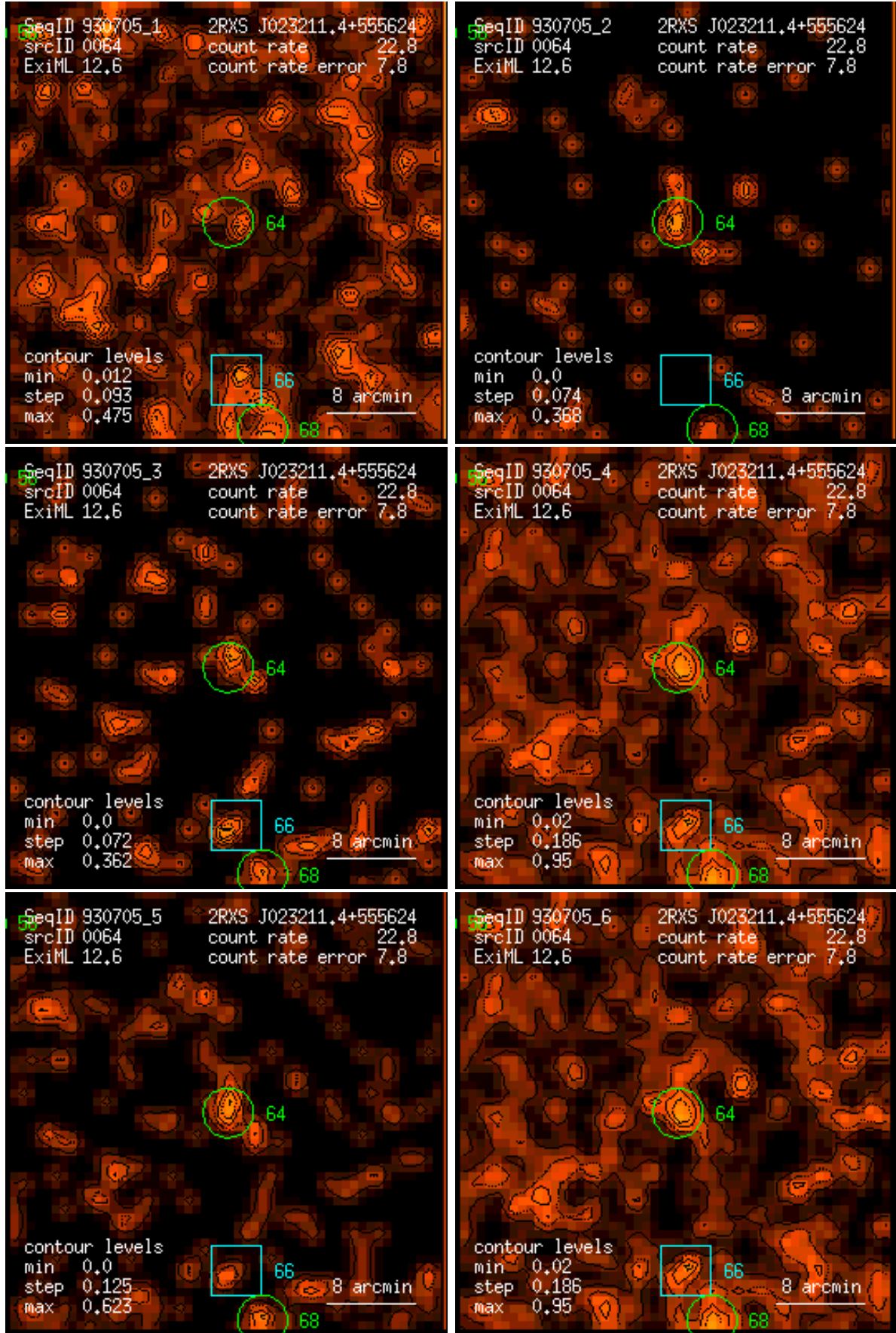
Figure 64: RASS 930705: detection 0064: band rate images, Gaussian filter: (1) PSPC channels 11 – 41, (2) 52 – 90, (3) 91 – 201, (4) 11 – 235, (5) 52 – 201, (6) 11 – 201. Broad band rates in counts/ks. Band rate contour levels in counts/ks/arcmin 2 .
