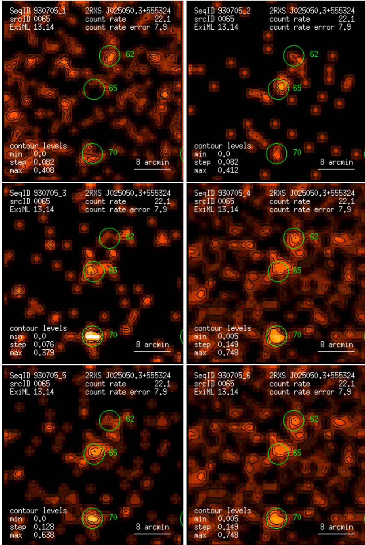
Figure 65: RASS 930705: detection 0065: band rate images, Gaussian filter: (1) PSPC channels 11 – 41, (2) 52 – 90, (3) 91 – 201, (4) 11 – 235, (5) 52 – 201, (6) 11 – 201. Broad band rates in counts/ks. Band rate contour levels in counts/ks/arcmin 2 .
