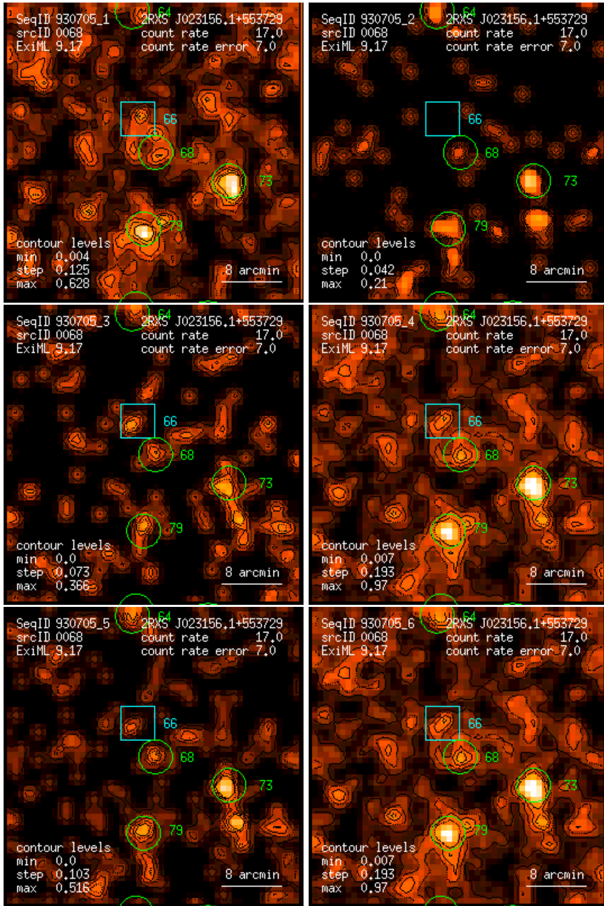
Figure 68: RASS 930705: detection 0068: band rate images, Gaussian filter: (1) PSPC channels 11 – 41, (2) 52 – 90, (3) 91 – 201, (4) 11 – 235, (5) 52 – 201, (6) 11 – 201. Broad band rates in counts/ks. Band rate contour levels in counts/ks/arcmin 2 .
