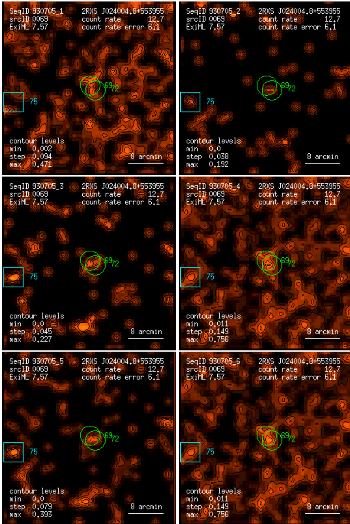
Figure 69: RASS 930705: detection 0069: band rate images, Gaussian filter: (1) PSPC channels 11 – 41, (2) 52 – 90, (3) 91 – 201, (4) 11 – 235, (5) 52 – 201, (6) 11 – 201. Broad band rates in counts/ks. Band rate contour levels in counts/ks/arcmin 2 .
