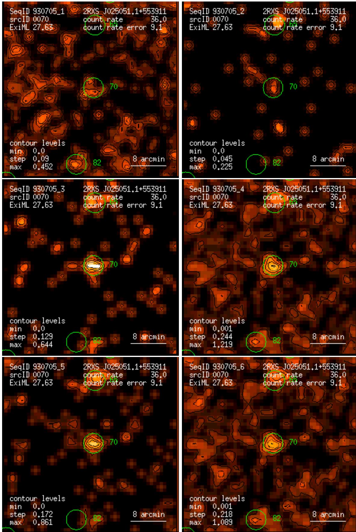
Figure 70: RASS 930705: detection 0070: band rate images, Gaussian filter: (1) PSPC channels 11 – 41, (2) 52 – 90, (3) 91 – 201, (4) 11 – 235, (5) 52 – 201, (6) 11 – 201. Broad band rates in counts/ks. Band rate contour levels in counts/ks/arcmin 2 .
