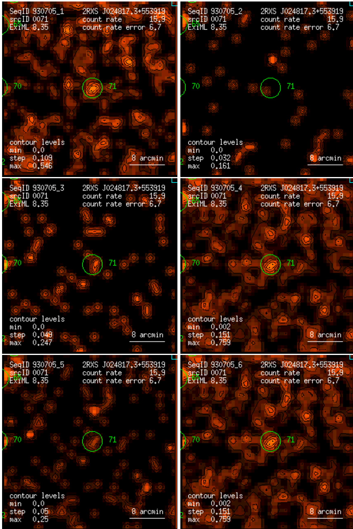
Figure 71: RASS 930705: detection 0071: band rate images, Gaussian filter: (1) PSPC channels 11 – 41, (2) 52 – 90, (3) 91 – 201, (4) 11 – 235, (5) 52 – 201, (6) 11 – 201. Broad band rates in counts/ks. Band rate contour levels in counts/ks/arcmin 2 .
