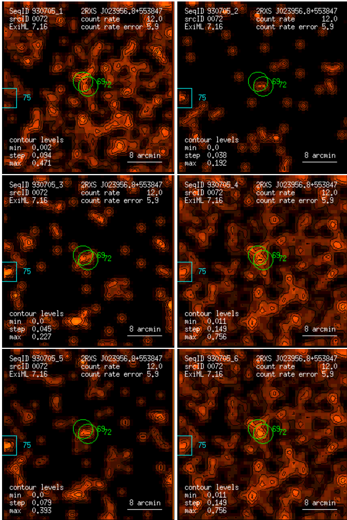
Figure 72: RASS 930705: detection 0072: band rate images, Gaussian filter: (1) PSPC channels 11 – 41, (2) 52 – 90, (3) 91 – 201, (4) 11 – 235, (5) 52 – 201, (6) 11 – 201. Broad band rates in counts/ks. Band rate contour levels in counts/ks/arcmin 2 .
