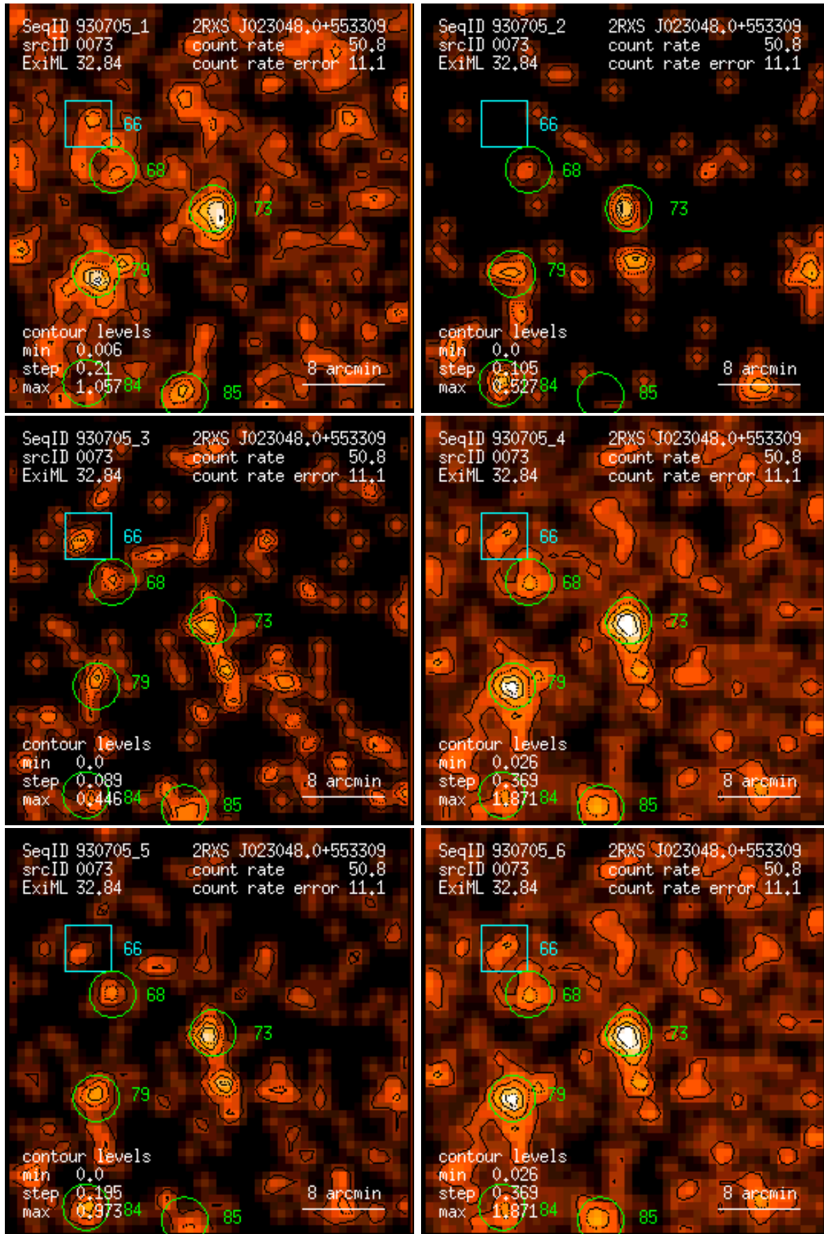
Figure 73: RASS 930705: detection 0073: band rate images, Gaussian filter: (1) PSPC channels 11 – 41, (2) 52 – 90, (3) 91 – 201, (4) 11 – 235, (5) 52 – 201, (6) 11 – 201. Broad band rates in counts/ks. Band rate contour levels in counts/ks/arcmin 2 .
