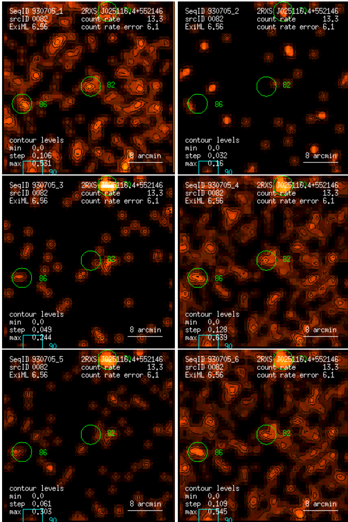
Figure 82: RASS 930705: detection 0082: band rate images, Gaussian filter: (1) PSPC channels 11 – 41, (2) 52 – 90, (3) 91 – 201, (4) 11 – 235, (5) 52 – 201, (6) 11 – 201. Broad band rates in counts/ks. Band rate contour levels in counts/ks/arcmin 2 .
