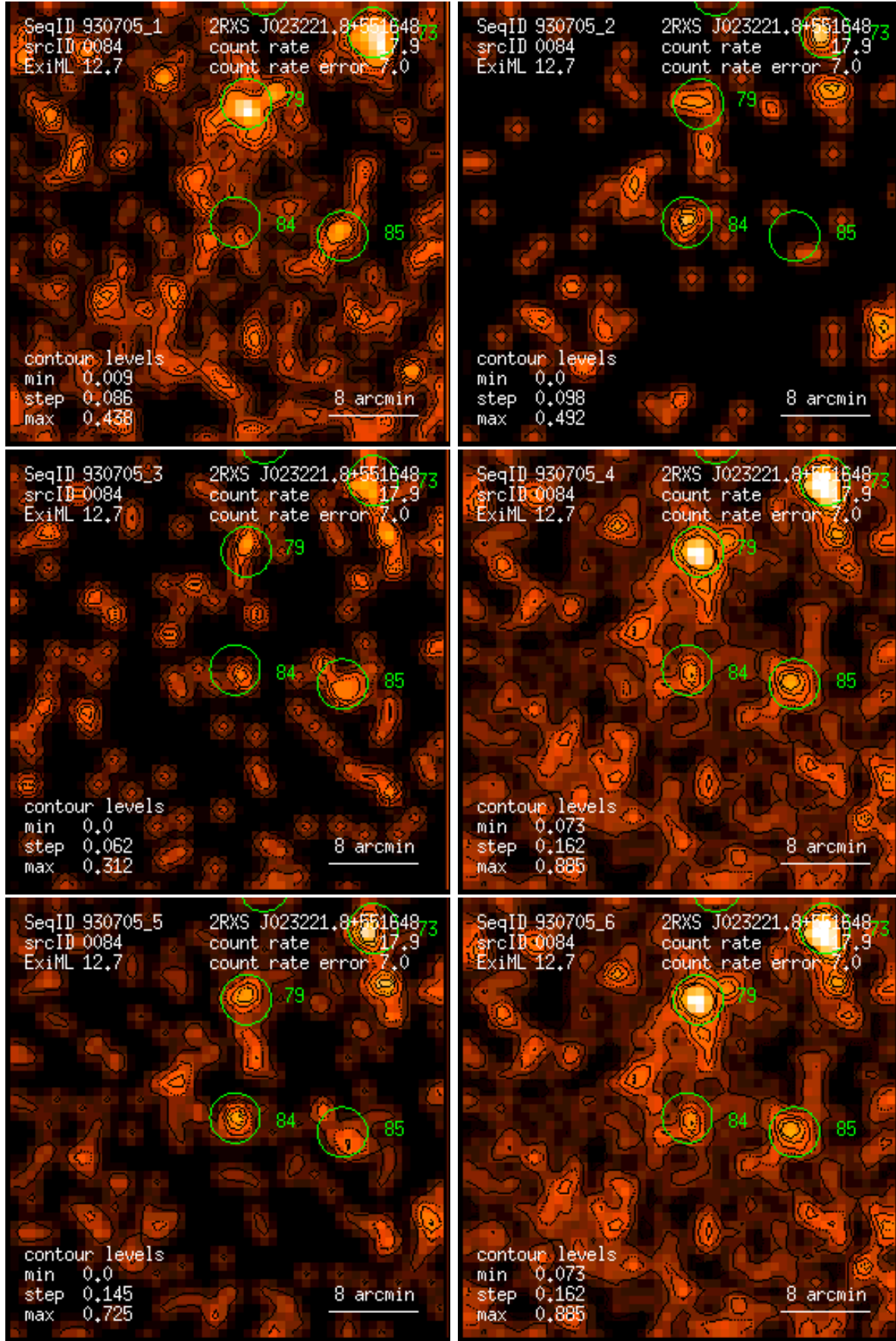
Figure 84: RASS 930705: detection 0084: band rate images, Gaussian filter: (1) PSPC channels 11 – 41, (2) 52 – 90, (3) 91 – 201, (4) 11 – 235, (5) 52 – 201, (6) 11 – 201. Broad band rates in counts/ks. Band rate contour levels in counts/ks/arcmin 2 .
