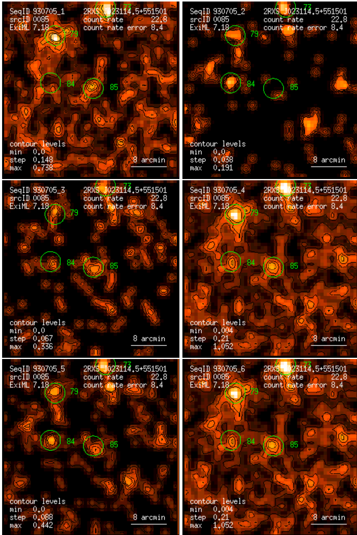
Figure 85: RASS 930705: detection 0085: band rate images, Gaussian filter: (1) PSPC channels 11 – 41, (2) 52 – 90, (3) 91 – 201, (4) 11 – 235, (5) 52 – 201, (6) 11 – 201. Broad band rates in counts/ks. Band rate contour levels in counts/ks/arcmin 2 .
